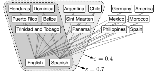
Figure 15: Case study 2: similar-bicliques in Unicode ( \tau = 2 )
