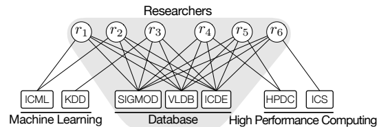
Figure 1: Example of researcher-venue bipartite graph
