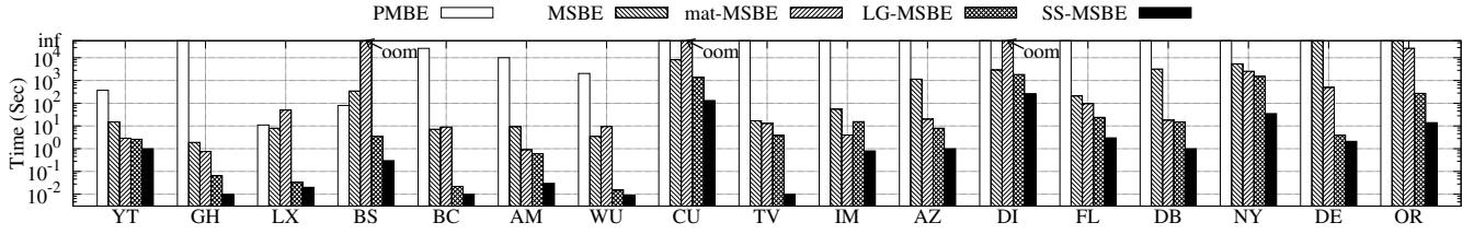
Figure 8: Running time on all graphs ( \epsilon = 0.5, \tau = 3 )
