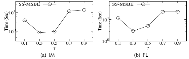
Figure 12: Efficiency of SS-MSBE by varying \gamma
