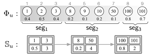
Figure 6: Example of consSS
