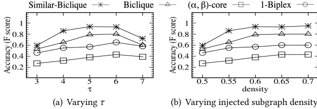
Figure 14: Case study 1: anomaly detection
