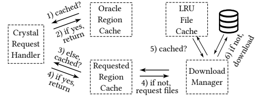
Figure 7: Request handling.
