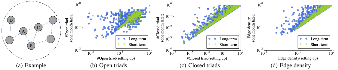
Figure 3: Group Structure Pattern. (a): An example of group friendship networks. Group members and friend relationships are represented as nodes and dot lines, respectively. For this example, we can see A, B and C are connected as a closed triad; A, C and D are connected as an open triad. The edge density of this group is 0.476. (b) (c): Horizontal axis is the normalized number of open/closed triads at the setting up of a WeChat group, and vertical axis is the normalized number of open/closed one month later. (c): Horizontal axis is the edge density at the setting up of a WeChat group, and vertical axis is the edge density one month later.
