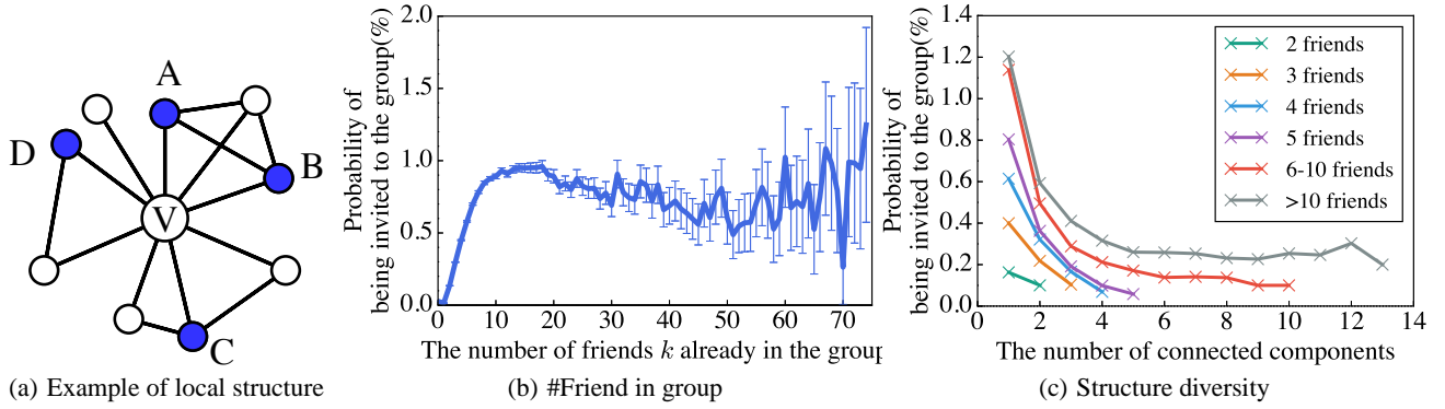
Figure 8: Local structure pattern of invitations. (a): Illustration of a potential invitee’s ego networks. Give a group \mathcal{C} , blue nodes represent user v ’s friends who have been in the group, while the white nodes denote those users in v ’s ego networks who did not join the group. (b): The probability p of being invited to a WeChat group as a function of the number of friends k already in the group. Error bars represent 95% confidence interval. (c): The effect of structure diversity. Structural diversity is represented by the number of connected components formed by the friends already in the group. Horizontal axis is the number of connected components formed by friends already in the group and the vertical axis is the probability p of being invited to a WeChat group.
