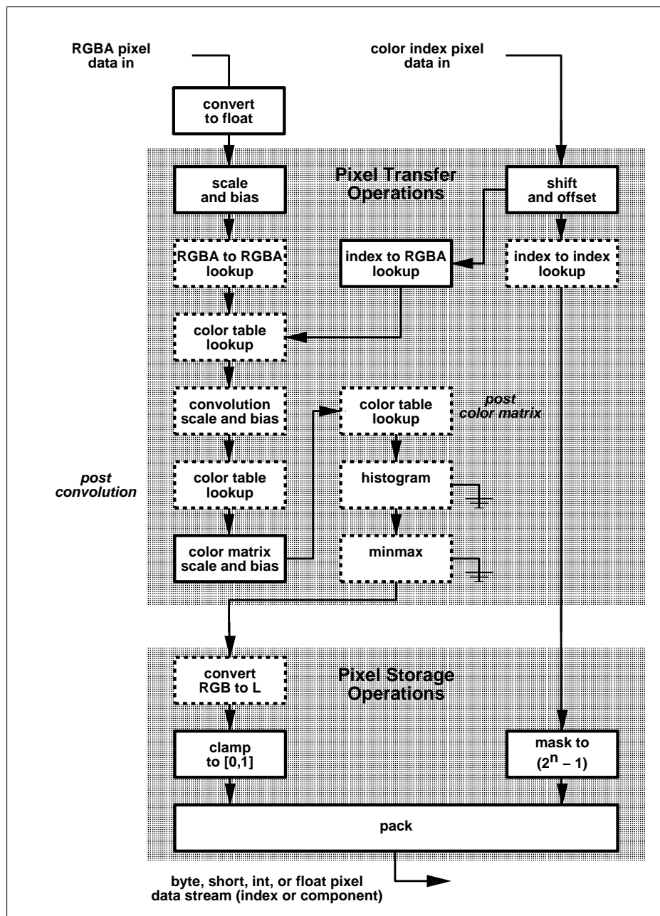
Figure 4.2. Operation of ReadPixels . Operations in dashed boxes may be enabled or disabled, except in the case of "convert RGB to L", which is only applied when reading color data in luminosity formats. RGBA and color index pixel paths are shown; depth and stencil pixel paths are not shown.
