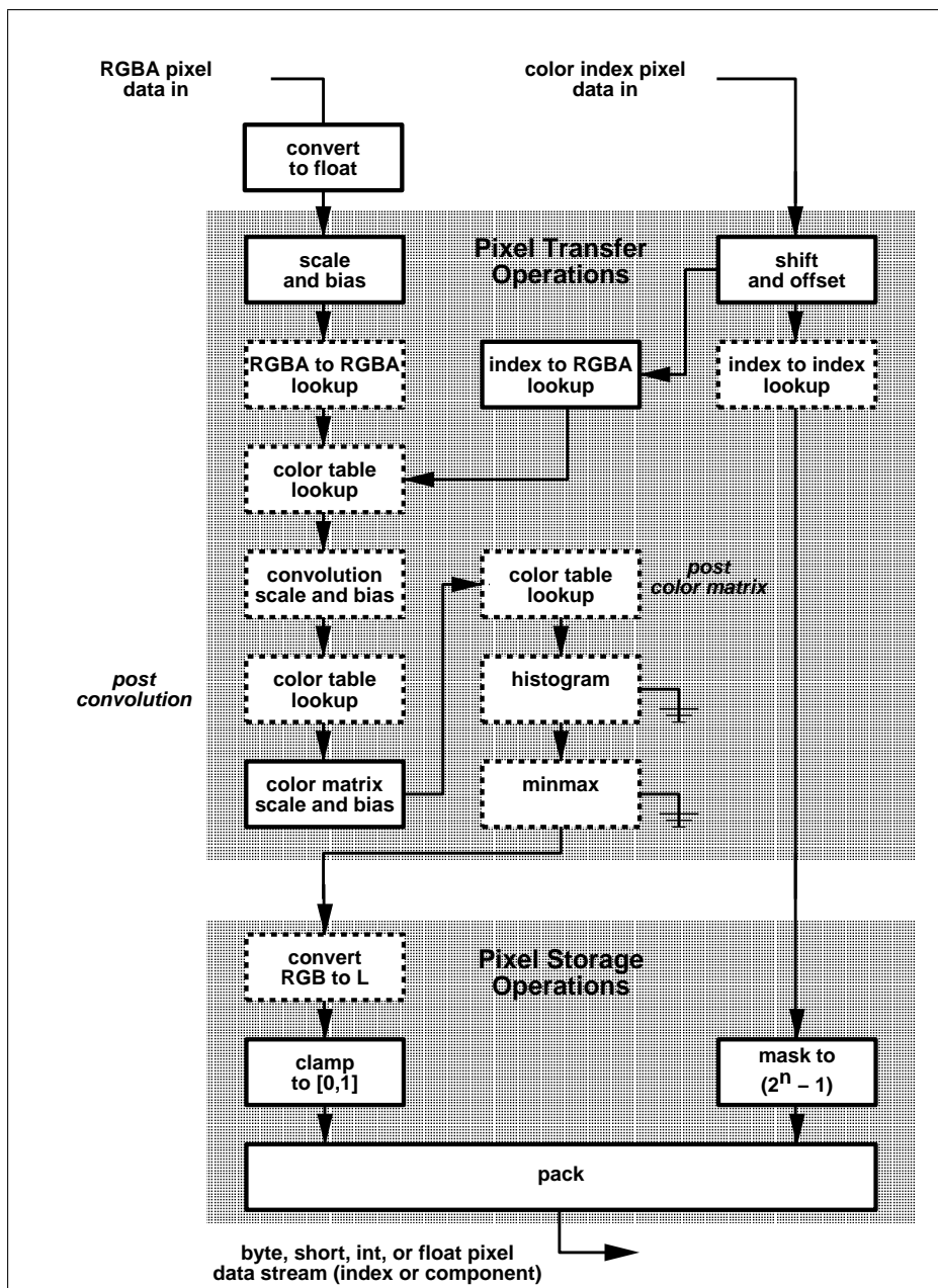
Figure 4.2. Operation of ReadPixels . Operations in dashed boxes may be enabled or disabled, except in the case of "convert RGB to L", which is only applied when reading color data in luminosity formats. RGBA and color index pixel paths are shown; depth and stencil pixel paths are not shown.
