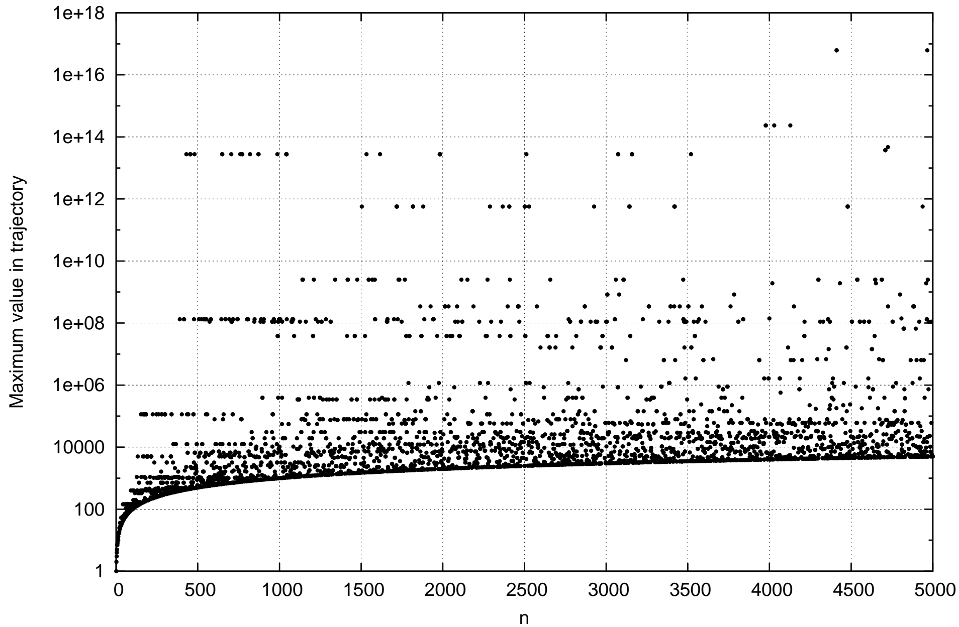
A291934, omitting conjecturally unbounded values
