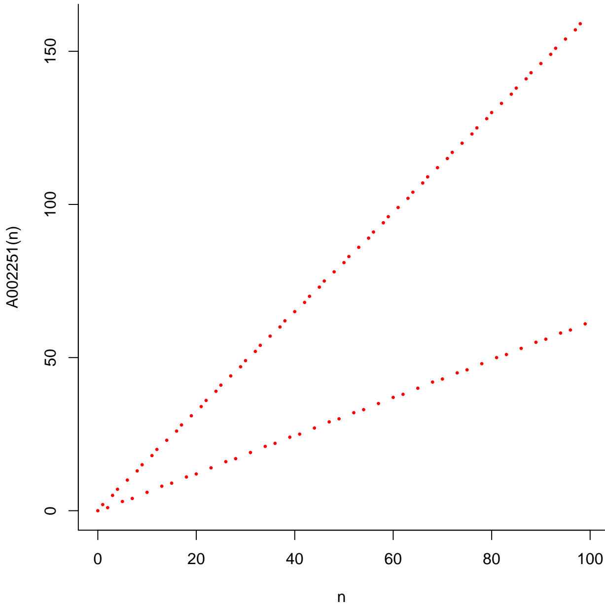
Scatterplot of A002251(n)
