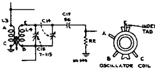
Oscillator Circuit RC-1046C, RC-1046E
