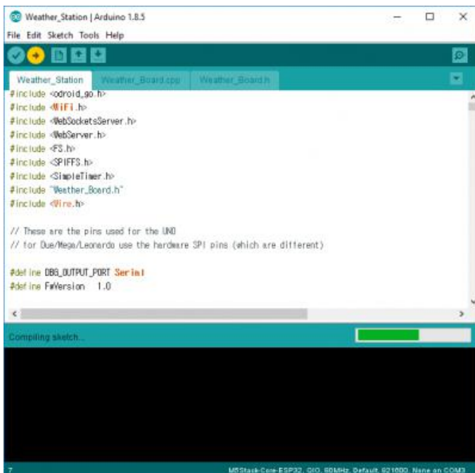
Figure 6 – Compiling Sketch
