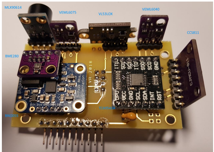
Figure 10 - Assembly Soldering
