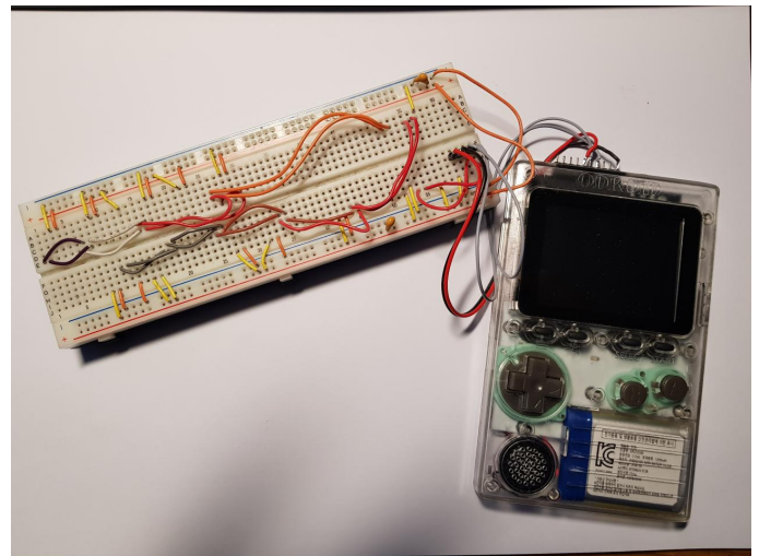
Figure 3 - Breadboard
