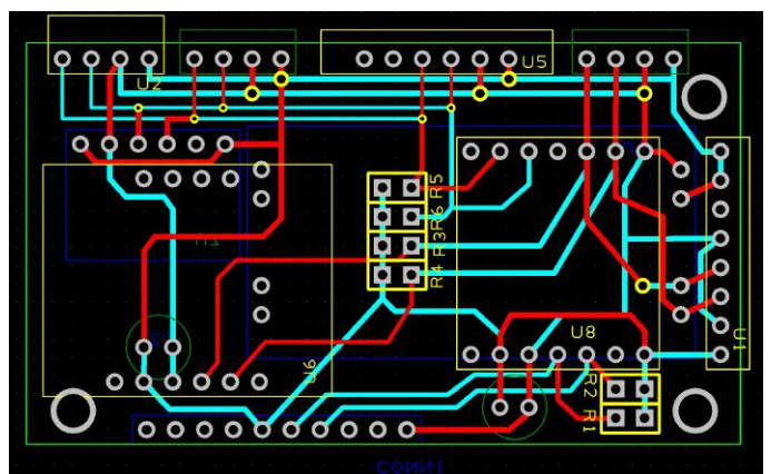
Figure 7 - PCB Layout
