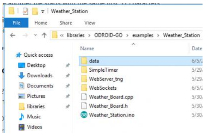
Figure 8 – data folder
