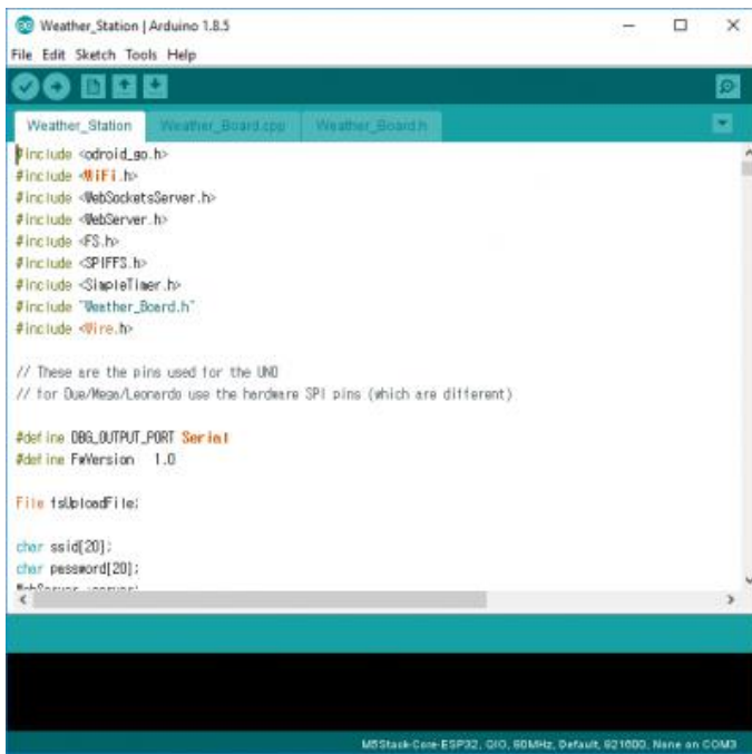
Figure 5 – Weather Code
