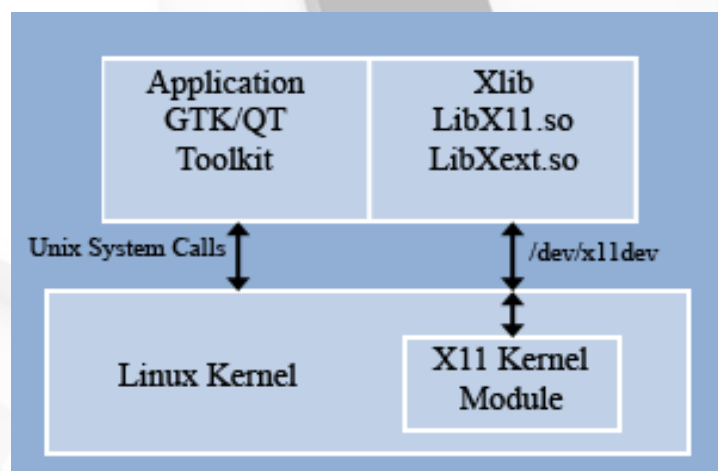
Figure 3 - MicroXwin
