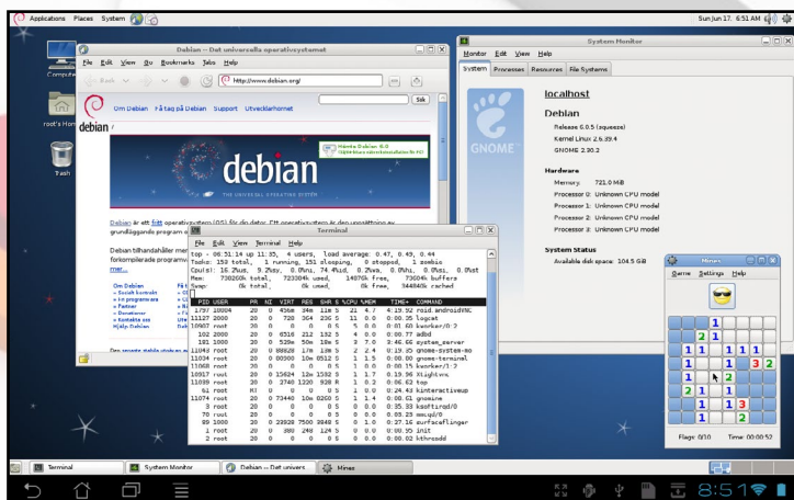
Figure 1 - Android-Debian
