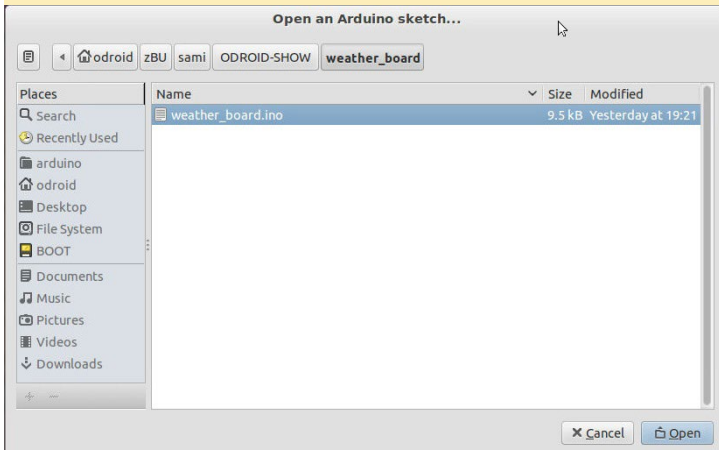
Figure 5: Open sketch
