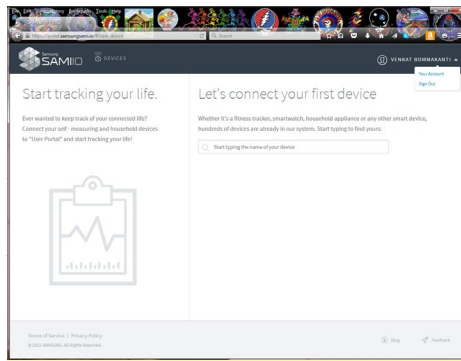
Figure 10: Post-login screen
