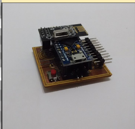
Figure 3- ProMicro unit
