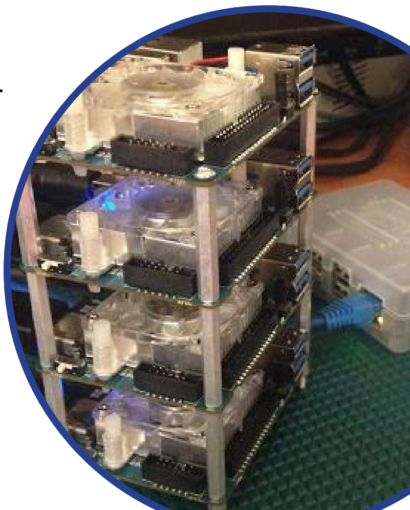
A XU4 cluster being managed by an XU3 console
