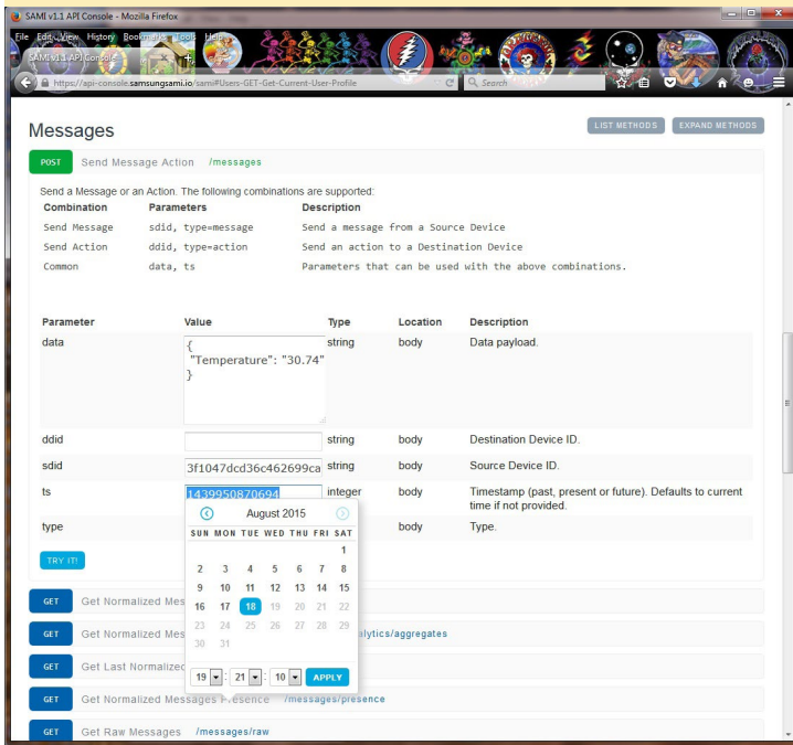
Figure 17: Messages API output
