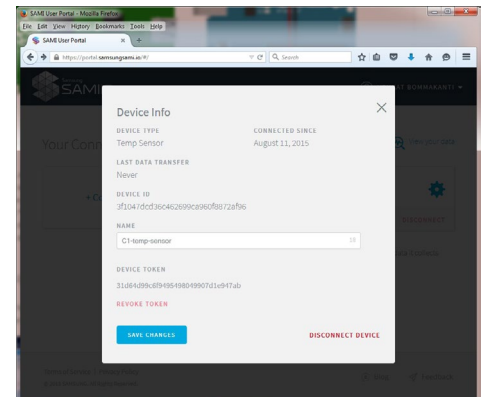
Figure 14: Device Token
