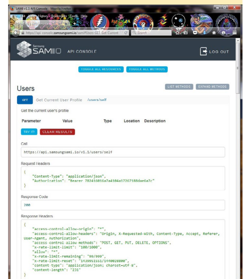
Figure 15: User information
