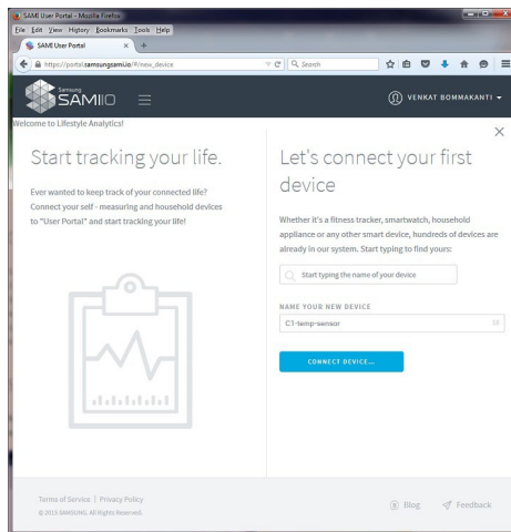
Figure 11: Device creation
