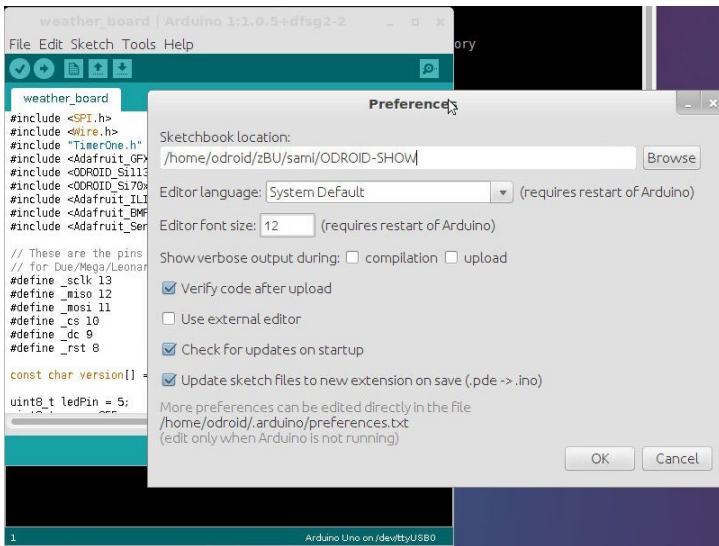
Figure 3: Arduino preferences
