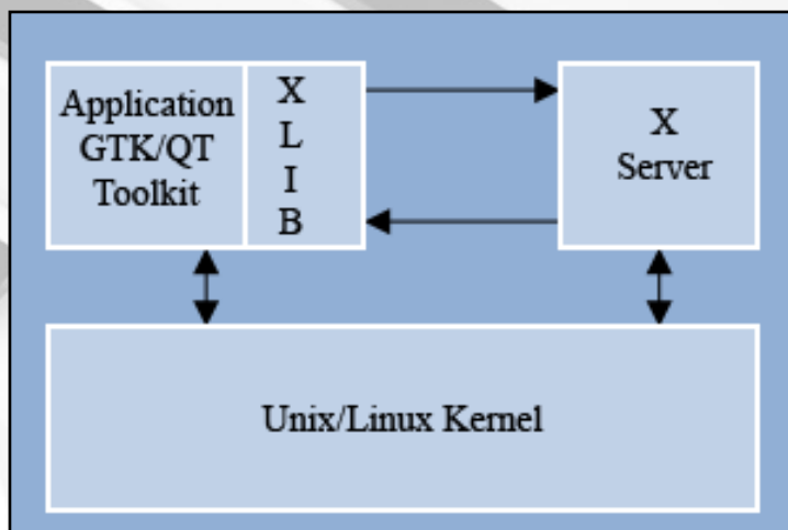
Figure 2 - X Windows
