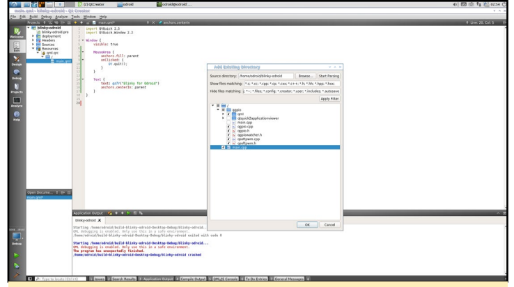
Figure 7 - Adding the QGPIO class to the project
