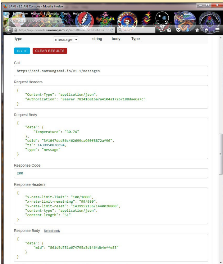
Figure 17: Messages API output
