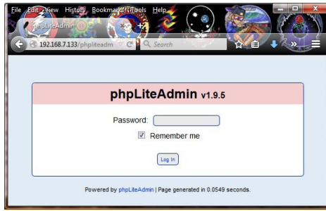
Figure 14 - phpLiteAdmin Login
