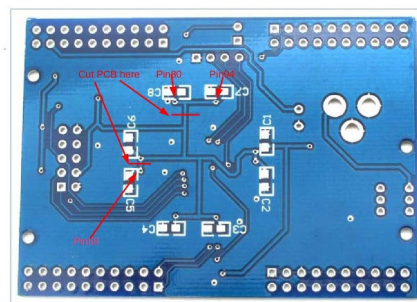
Figure 4 - PCB modifications
