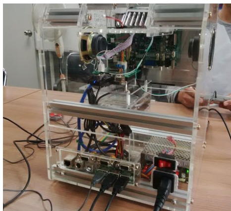
Figure 13 - Rear view
