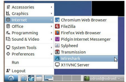
Figure 5 - Launch Wireshark
