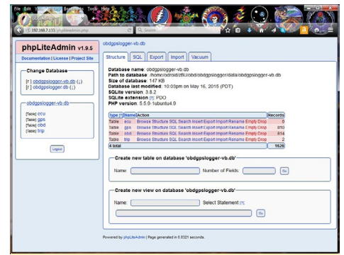
Figure 15 - phpLiteAdmin welcome
