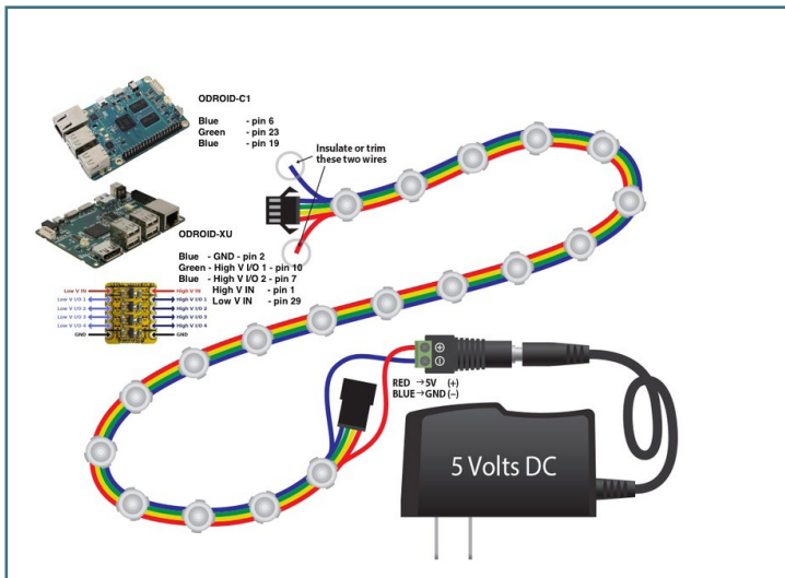
Figure 2 - Connection diagram
