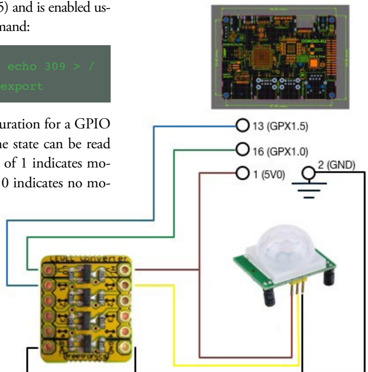
Connect the Motion Sensor as show in this schematic, remember that this is for the ODROID-XU
