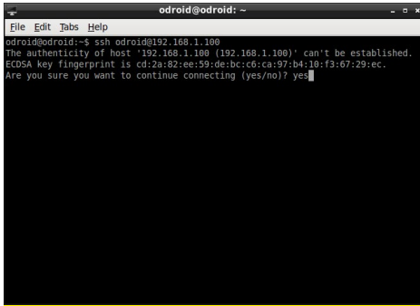
Establishing an SSH connection to our server
