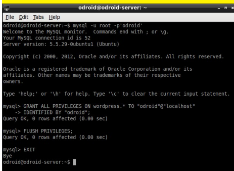
Configuring the MySQL server for use by WordPress
