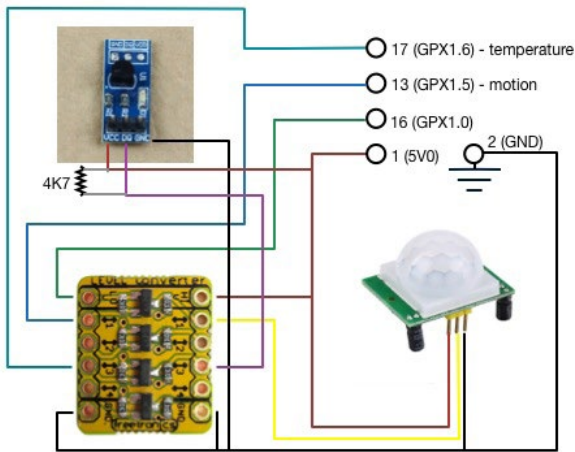
Connect the Temperature Sensor
