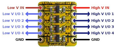
Freertronics Logic Level Converter Module with 4 IO Ports
