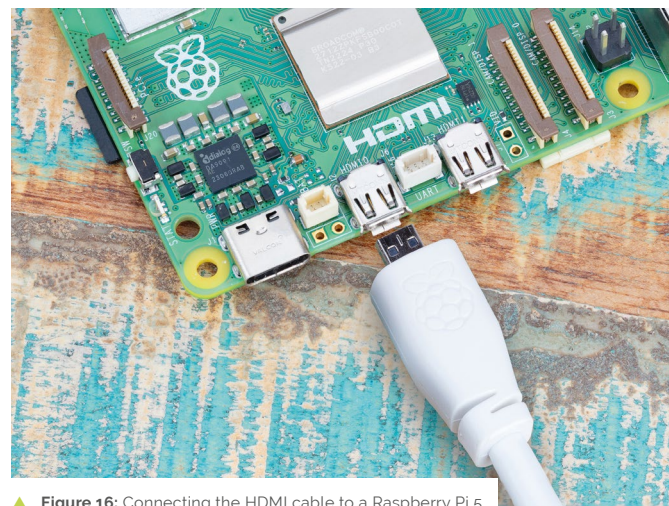
▲ Figure 16: Connecting the HDMI cable to a Raspberry Pi 5
