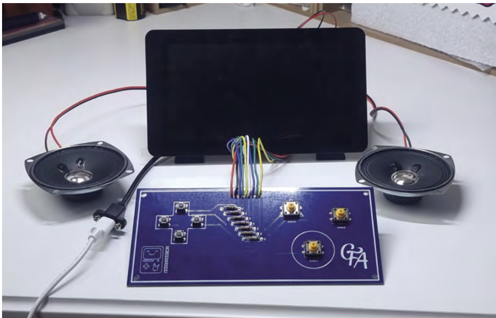
▼ The PCB for this project was custom-made by Geeky Faye
