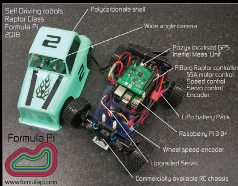
Above You can paint your Raptor's shell, as well as write its controlling code
