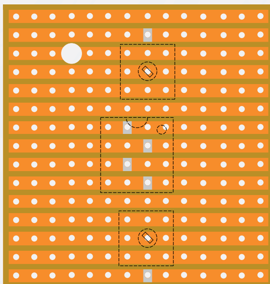
Figure 3 Top trace, left controller; bottom trace, right controller
