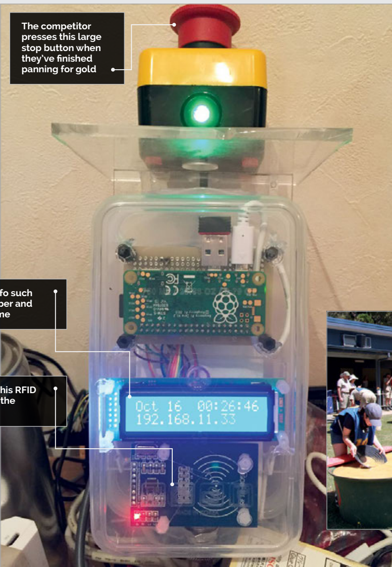
Above Daryl's new timers were a big hit with competitors, who had greater confidence in the times recorded
