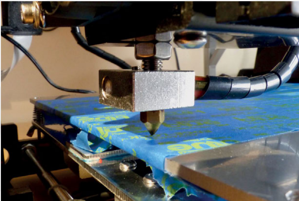
Above Levelling is one of the most important parts of successful 3D printing. Too high, the filament won't stick. Too low, you risk damage to your printer
