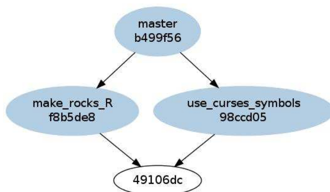
Figure 3: The repo history after our second merge.
