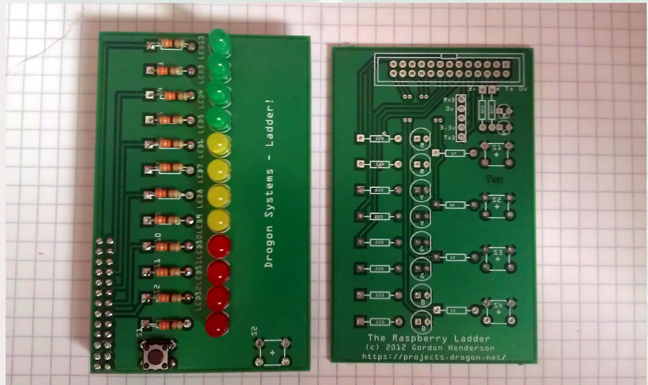
Prototype Raspberry Ladder Board and PCB
