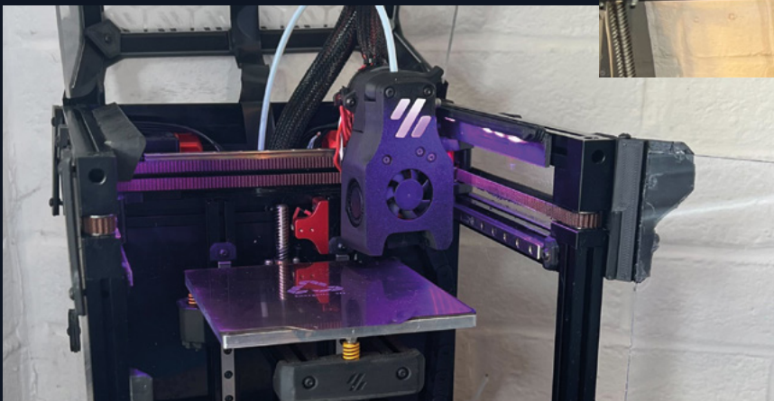
Left ◀ Each belt loops around both the Y and X axes
