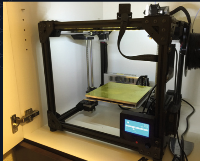
Above ↕ The first Voron prototype
