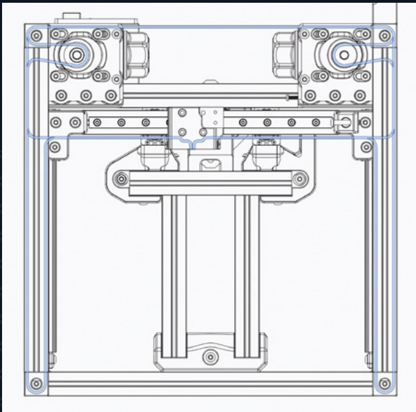
Left ◀ It can be a bit tricky to follow the belt path, but the key thing is that both motors stay still while the print head moves
