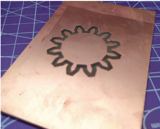
Figure 2 ♦ Etching a gear design into copper using a vinyl mask and ferric chloride
