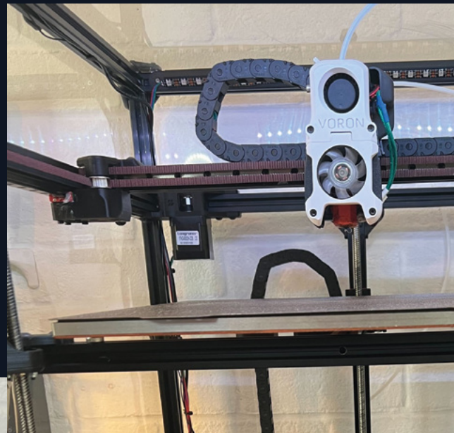
Left ◀ It can be a bit tricky to follow the belt path, but the key thing is that both motors stay still while the print head moves
