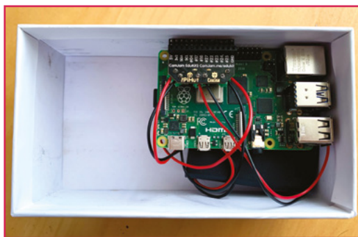
▲ You can use the battery pack and Raspberry Pi 4 as 'ballast' at the rear. Add a power bank for true remote computing!
