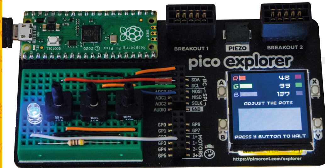
Below The complete circuit, with an LED and three potentiometers
