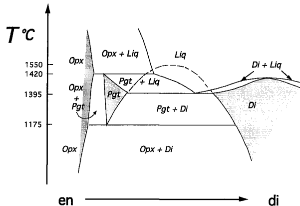
FIGURE 2. Schematic temperature-composition relations for the En-Di join at 1 atm, excluding equilibria that involve protoenstatite and Fo but including liquidus equilibria (some metastable). Dashed curve is the metastable portion of the Pgt-Di solvus. Temperatures are extrapolated from Figure 1 of Longhi and Boudreau (1980) and from Figure 2 of Carlson and Lindsley (1988), as explained in the text.
