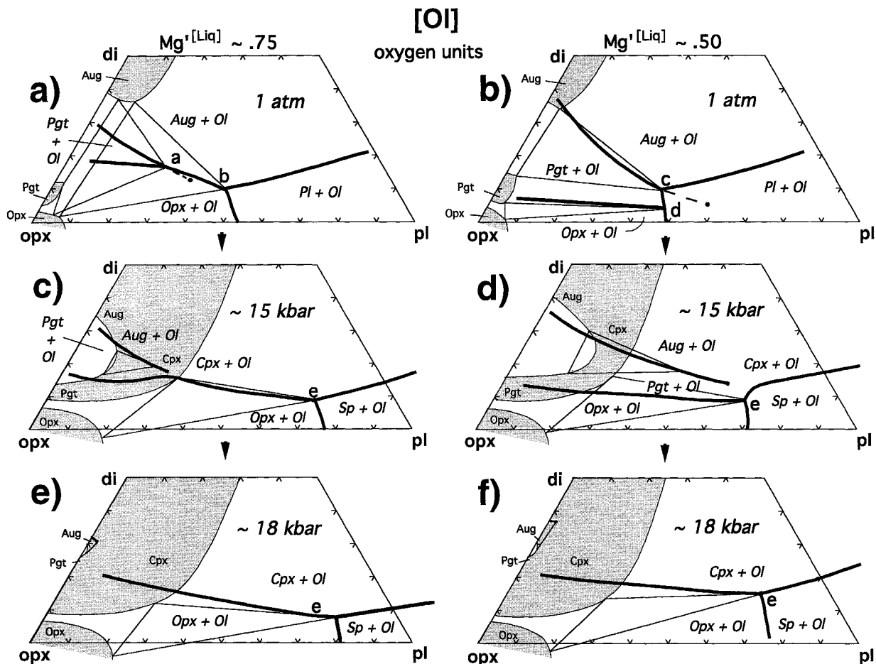
FIGURE 6. Schematic progression of liquidus boundaries and pyroxene solid-solution fields with pressure on the Ol saturation surface. Heavy curves are liquidus boundaries; light solid lines are tielines joining compositions of coexisting phases; shaded areas are polythermal fields of stable pyroxene composition. The letters a, b, c, and d refer to the same pseudounivariant equilibria
