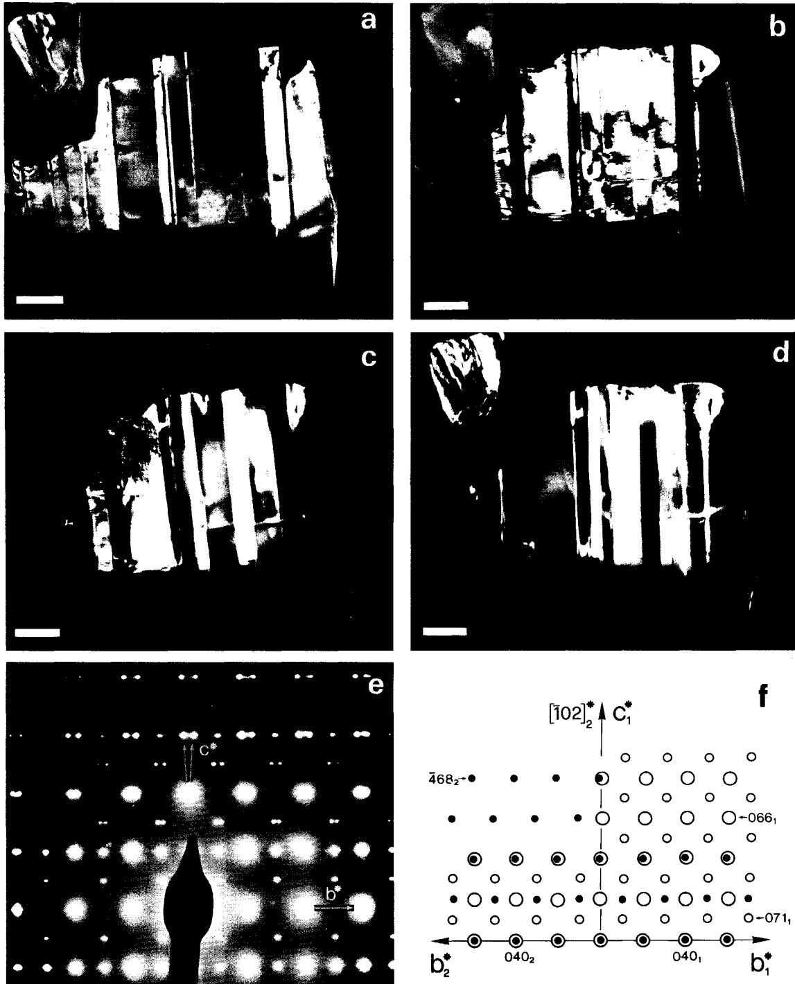
Fig. 2. \text{SrF}_{80}\text{An}_{20} sample ( T = 1350^\circ\text{C} , t = 456\text{ h} + T = 1530^\circ\text{C} , t = 2\text{ h} ). Dark-field images of albite and Carlsbad twins; scale bar: 0.2\ \mu\text{m} . (a and b) Carlsbad-twinned individuals, g = 152_2 and g = 062_1 . In b, composition planes normal to (010) and tweed textures are observed. (c and d) Albite twins within the Carlsbad individual visible in b, g = 006_{1a} and g = 006_{1b} . (e) SAD pattern from the same grain. Note streaking parallel to
