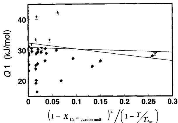
Fig. 1. Regular-solution interpretation of calcite-saturated liquidus in \text{CaCO}_3\text{-BaSO}_4\text{-CaF}_2 (500 bars \text{CO}_2 , Kuellmer et al., 1966), following Eq. 12. See Table 3 for definition of Q1 . Open and filled symbols represent liquid-only and liquid + calcite experiments, respectively. Lines from each data point represent a conservative estimate of errors ( \pm 5 K in T ; \pm 0.2 wt% in X ), showing only the error bar halves that contribute to uncertainty in slope and intercept. The liquidus surfaces, linear with slope W and ordinate intercept of \Delta\bar{H}_{\text{fus}}^0(\text{calcite}) , should lie between these groups of experiments. Within error, all data are consistent with \Delta\bar{H}_{\text{fus}}^0(\text{calcite}) = 31.5 \pm 1 kJ/mol and W_{\text{Ca}^{2+}\text{-Ba}^{2+}} = -11 \pm 9 kJ/mol 2 (thin solid lines).
