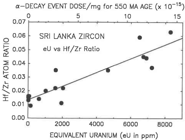
Fig. 1. Hf/Zr atom ratio for Sri Lanka gem zircon samples, measured by electron microprobe, as a function of equivalent U (eU) measured by scintillation counter. Calculated total \alpha -decay event dosage based on a 550 Ma age for Sri Lanka gem zircon samples is shown across the top. The linear regression best fit to the data is shown; \text{Hf/Zr} = 0.013 + 5 \times 10^{-6} \text{ eU} , r^2 = 0.83 .
