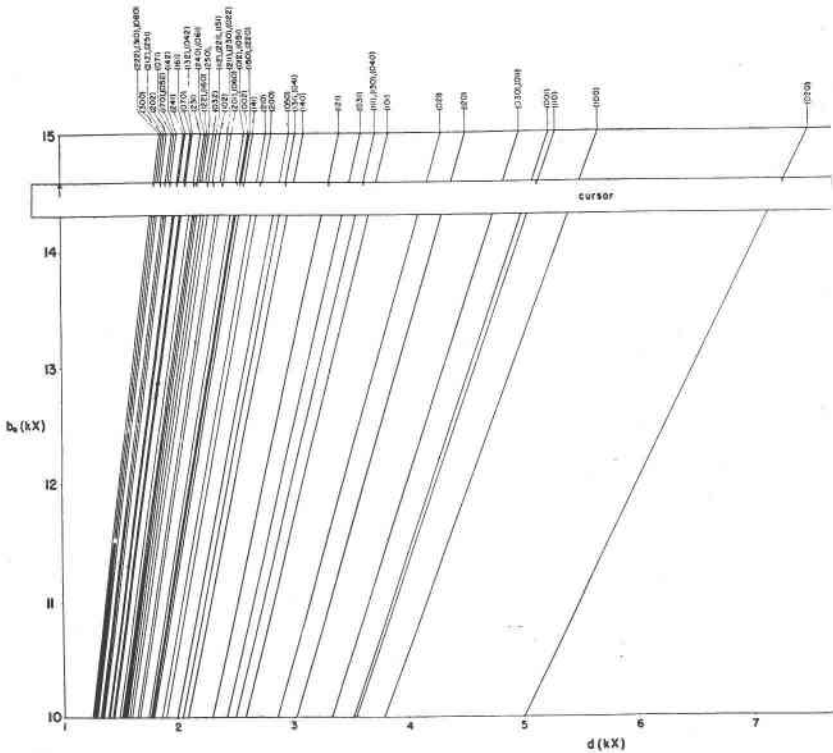
FIG. 7. Analyzer for euxenite giving the variations of d(hkl) with b for the morphological ratio a:b:c=0.3789:1:0.3527 .
