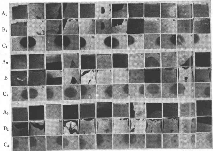
FIG. 1. Photographs of quartz plates etched to show twin pattern before (A) and after (B) heating through the inversion temperature ( 573^{\circ} \pm 1^{\circ} C) and of the same plates after irradiation (C).
