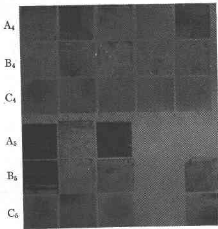
FIG. 2. Photographs of quartz plates etched to show twin pattern before (A) and after (B) heating through the inversion temperature ( 573^{\circ} \pm 1^{\circ} C) and of the same plates after irradiation (C).
