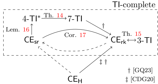
Figure 1: Reduction between problems and TI-completeness. “ A \rightarrow B ” indicates that A reduces to B . Dashed arrows denote trivial reductions.
