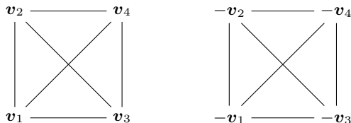
Fig. 2: The graph of the class C_4
