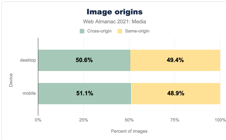
Figure 5.26. Image origins.
