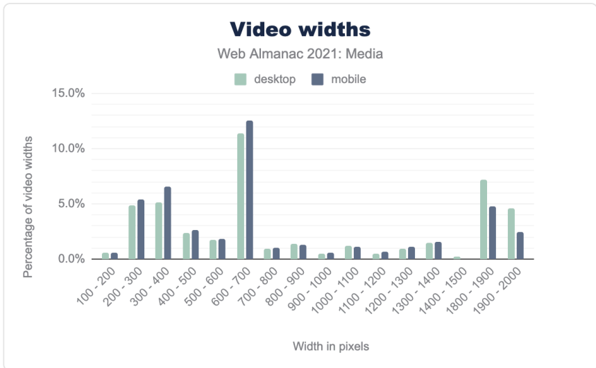
Figure 5.33. Video widths.
