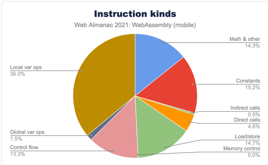
Figure 6.21. Instruction kinds.
