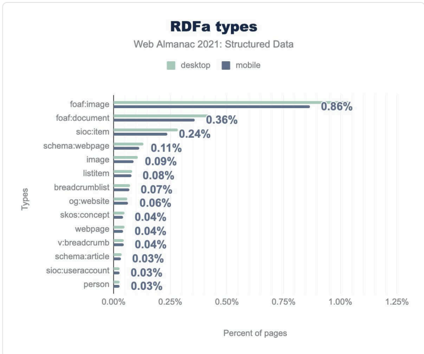
Figure 4.2. RDFa types
