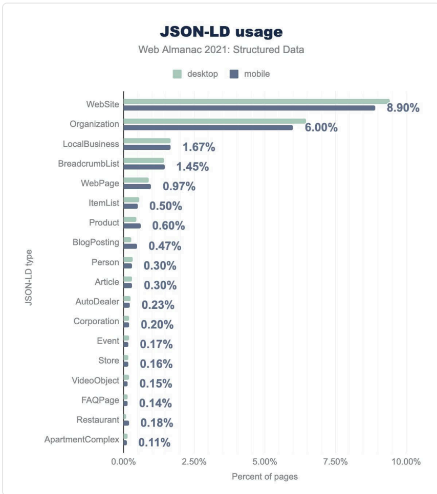
Figure 4.14. SameAs usage
