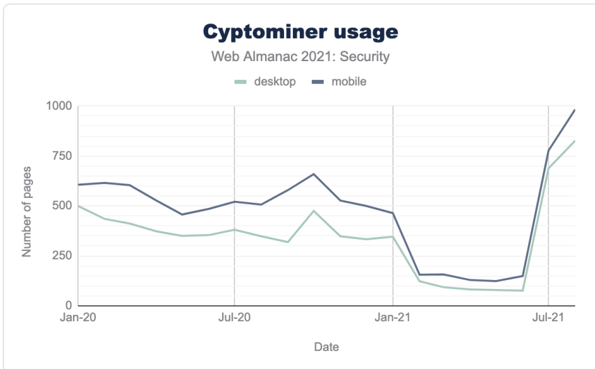
Figure 12.34. Cryptominer usage.
