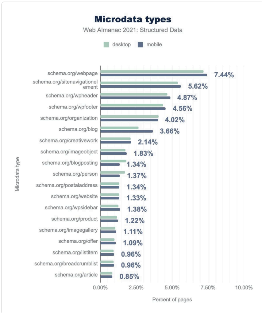
Figure 4.9. Microdata types
