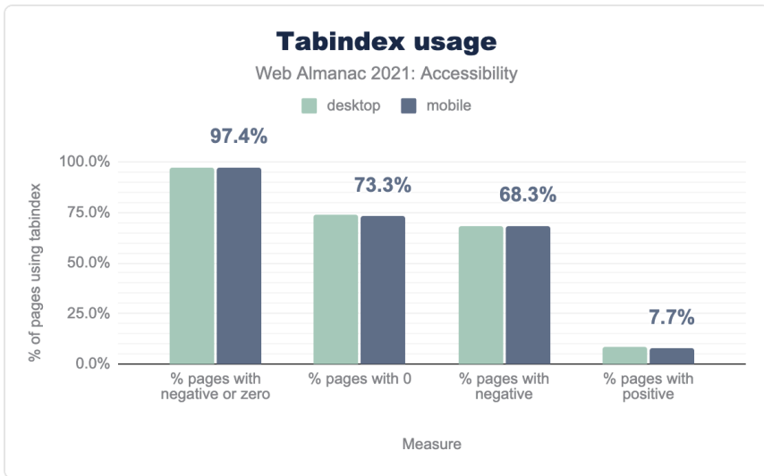
Figure 9.10. tabindex usage
