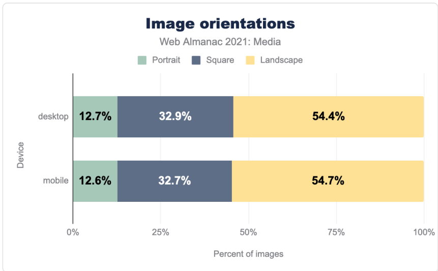
Figure 5.9. Image orientations.
