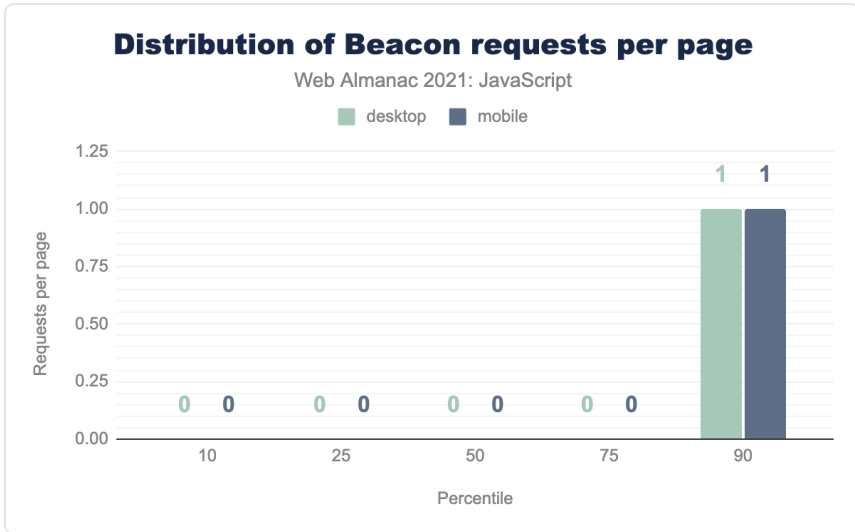
Figure 2.35. Distribution of the number of Beacon requests per page.
