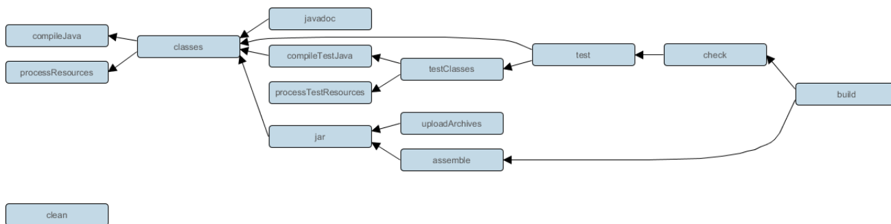
Figure 34. Java plugin - tasks
