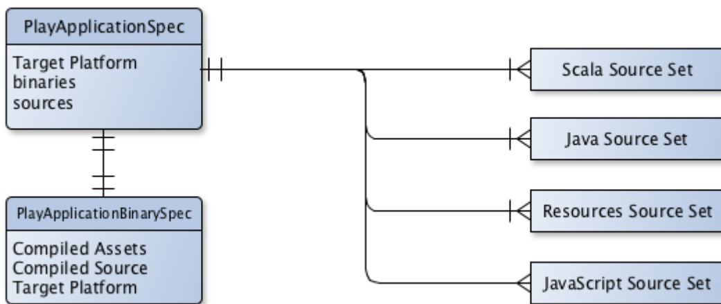
Figure 32. Play plugin - software model
