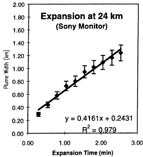
Figure 1-5. Plume width at an altitude of 24 km as a function of expansion time.
