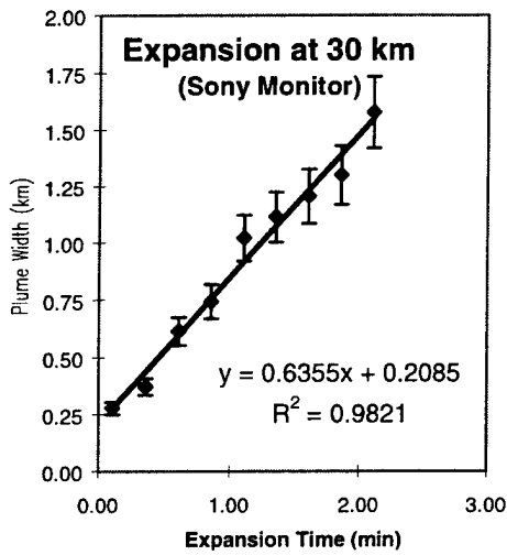
Figure 1-6. Plume width at an altitude of 30 km as a function of expansion time.
