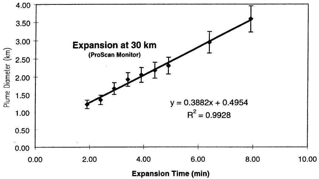
Figure 5-6. Plume width as a function of expansion time from Haulover Canal taken with the camera assigned to observe the plume at an altitude of 30 km.
