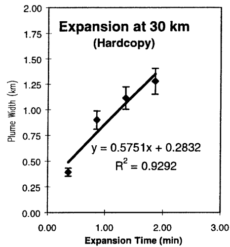
Figure 1-6. Plume width at an altitude of 30 km as a function of expansion time.
