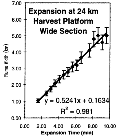
Figure 2-6. Plume width at an altitude of 24 km from Harvest as a function of expansion time.
