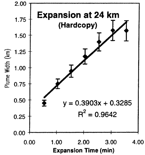
Figure 1-5. Plume width at an altitude of 24 km as a function of expansion time.
