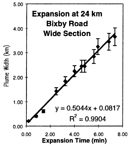
Figure 2-7. Plume width at an altitude of 24 km as a function of expansion time.
