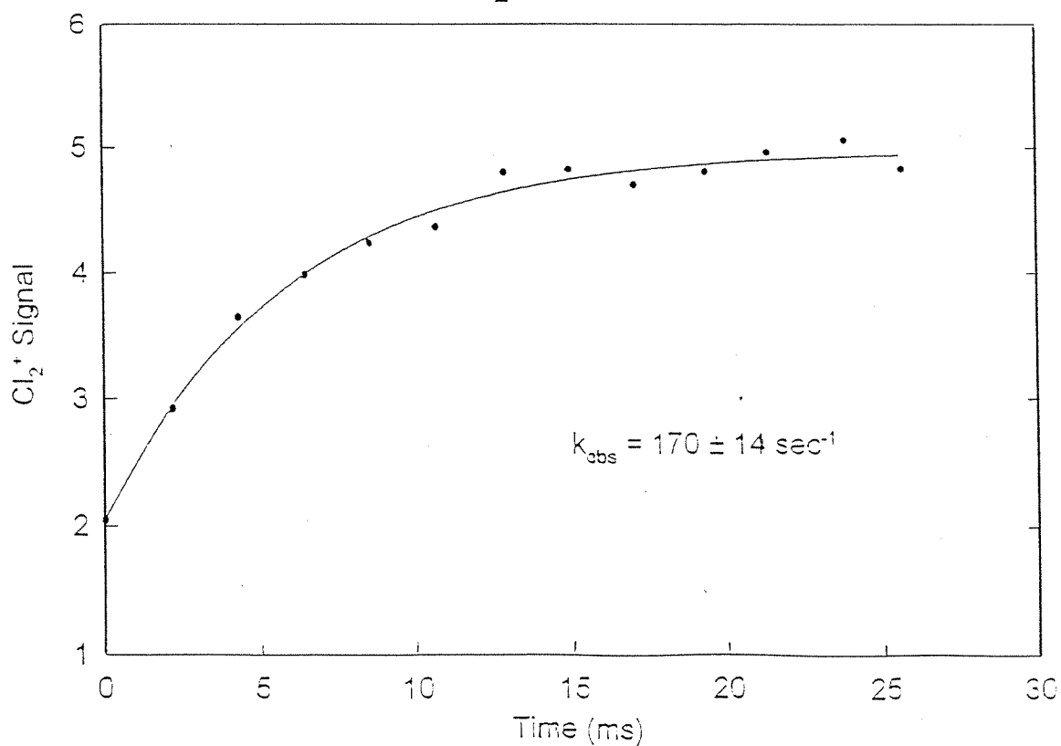
Figure 1. [ClONO 2 ] = 7.54 × 10 -7 Torr, [HCl] = 7.46 × 10 -6 Torr, [H 2 O] = 4.81 × 10 -4 Torr
