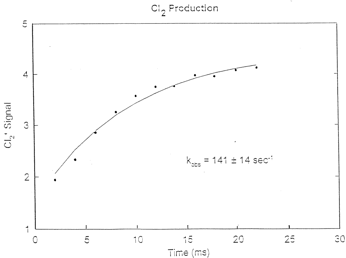
Figure 3. [ClONO 2 ] = 7.56 × 10 -7 Torr, [HCl] = 8.33 × 10 -6 Torr, [H 2 O] = 4.41 × 10 -4 Torr
