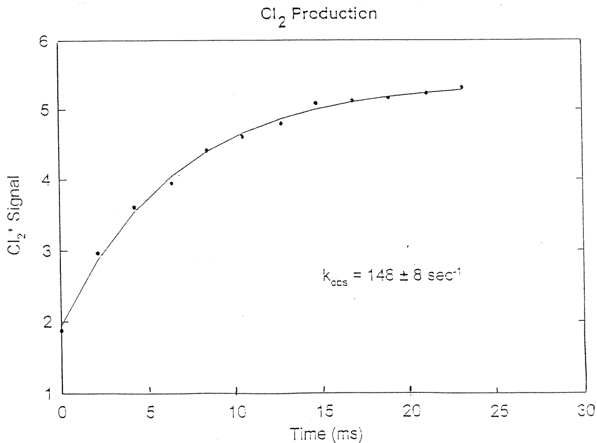
Figure 2. [ClONO 2 ] = 7.81 × 10 -7 Torr, [HCl] = 7.71 × 10 -6 Torr, [H 2 O] = 4.57 × 10 -4 Torr
