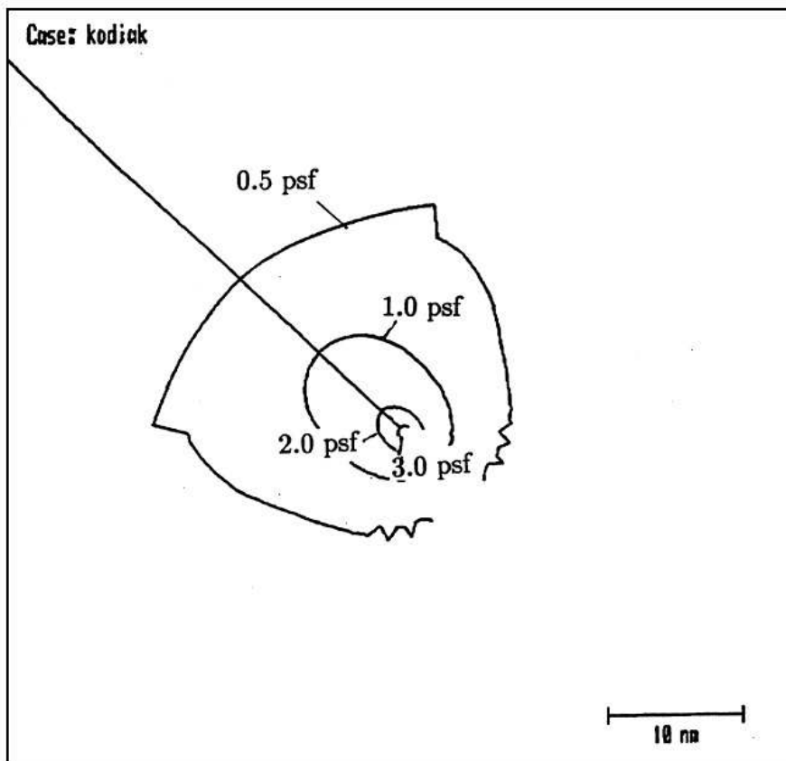
Figure 6: Overpressure Foot Print: Descent Boom (from K. Plotkin)
