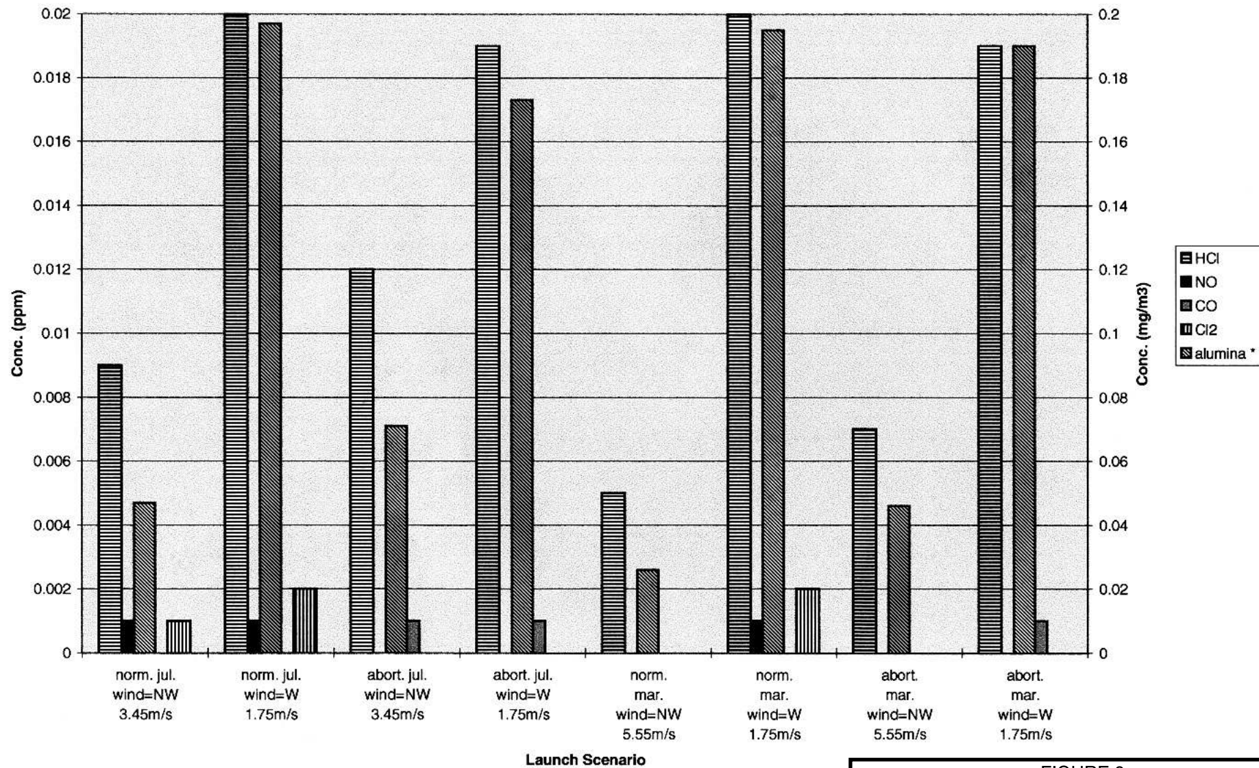
FIGURE 9 MAXIMUM 60 MINUTE MEAN CONCENTRATIONS VS. LAUNCH SCENARIO
