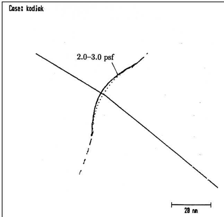
Figure 5: Overpressure Foot Print: Kodak Ascent Boom (from K. Plotkin)
