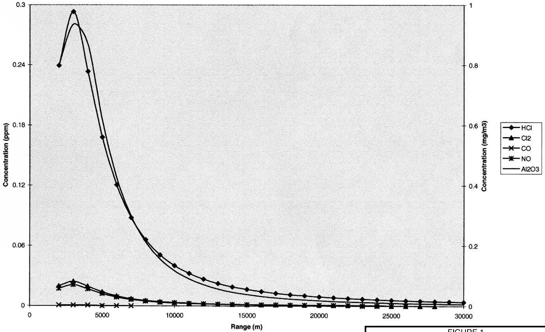
FIGURE 1 DOWNWIND CONCENTRATIONS FROM NORMAL JULY LAUNCH OF AIT, PREVAILING WIND CONDITIONS
