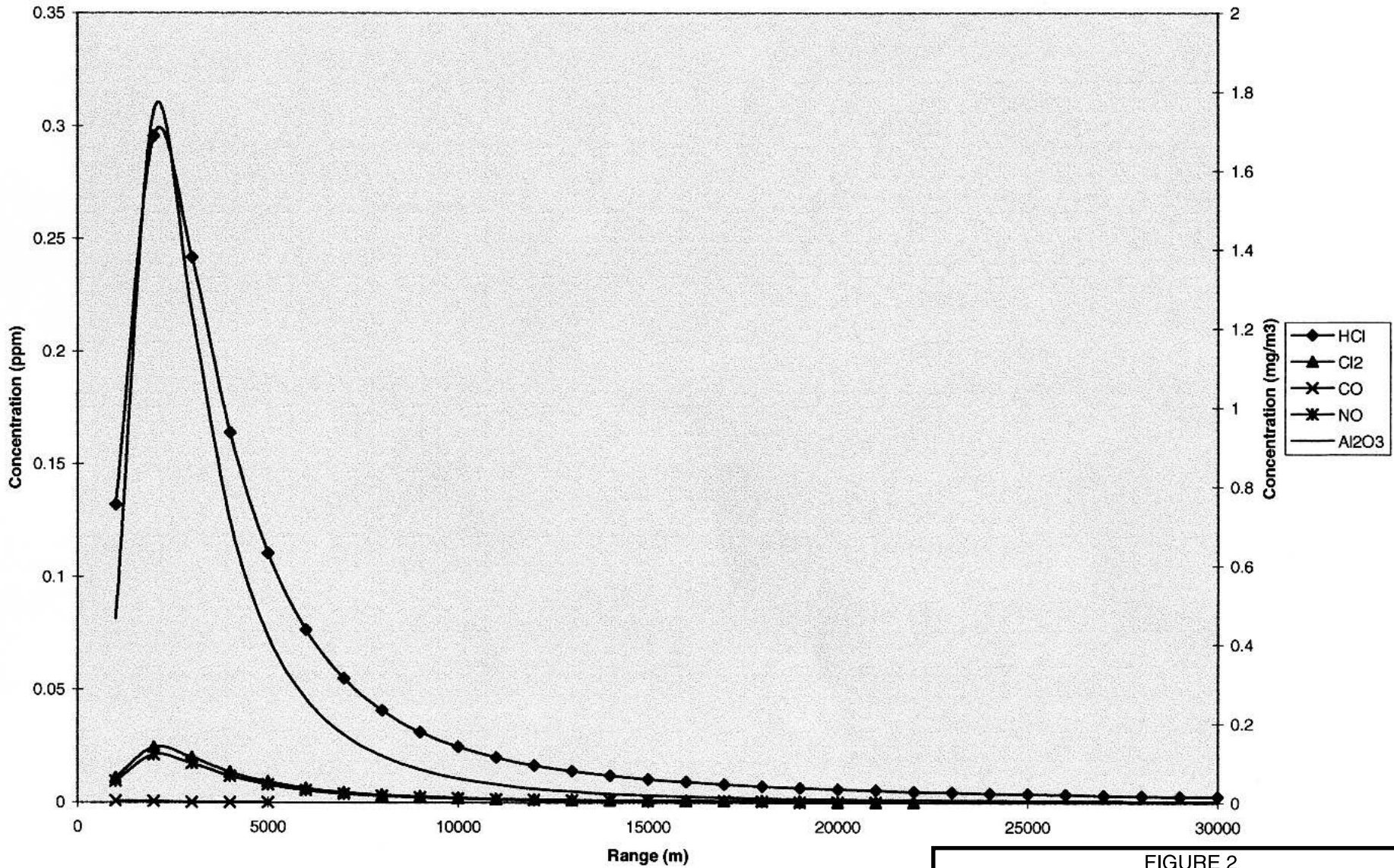
FIGURE 2 DOWNWIND CONCENTRATIONS FROM NORMAL JULY LAUNCH OF AIT, CALM WIND CONDITIONS
