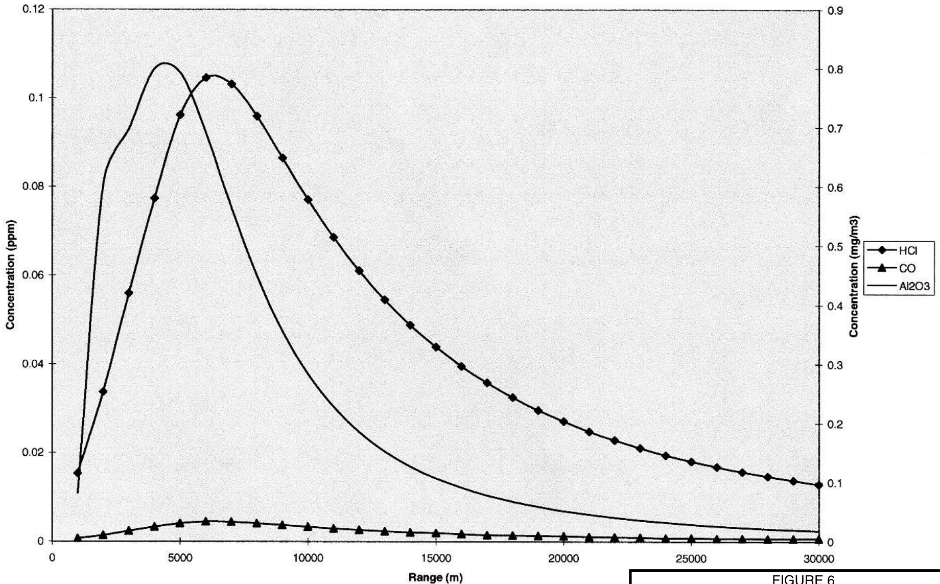
FIGURE 6 DOWNWIND CONCENTRATIONS FROM ABORT OF JULY LAUNCH OF AIT, CALM WIND CONDITIONS
