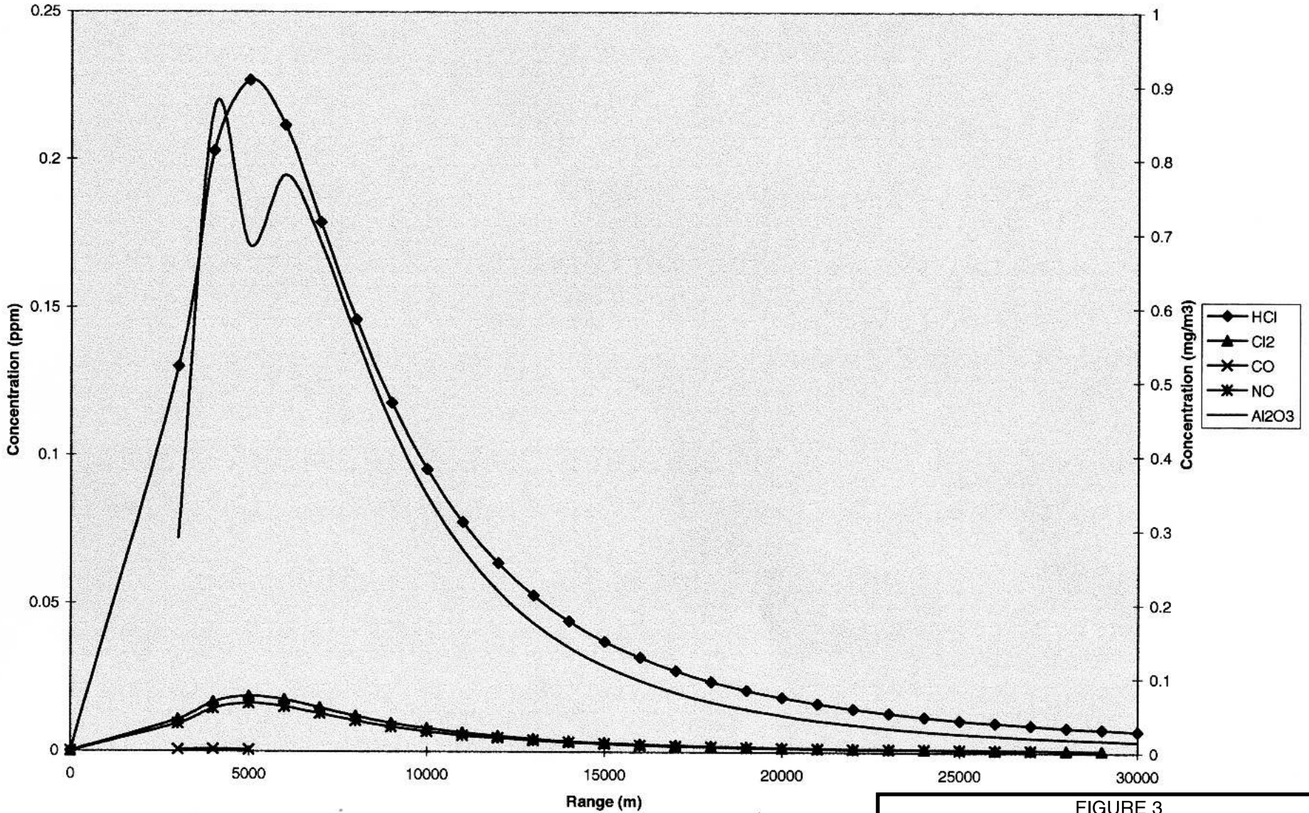
FIGURE 3 DOWNWIND CONCENTRATIONS FROM NORMAL MARCH LAUNCH OF AIT, PREVAILING WIND CONDITIONS
