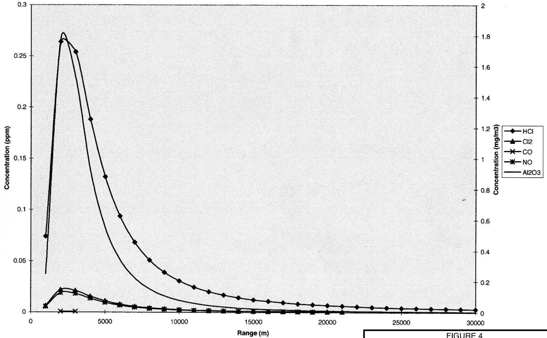
FIGURE 4 DOWNWIND CONCENTRATIONS FROM NORMAL MARCH LAUNCH OF AIT, CALM WIND CONDITIONS
