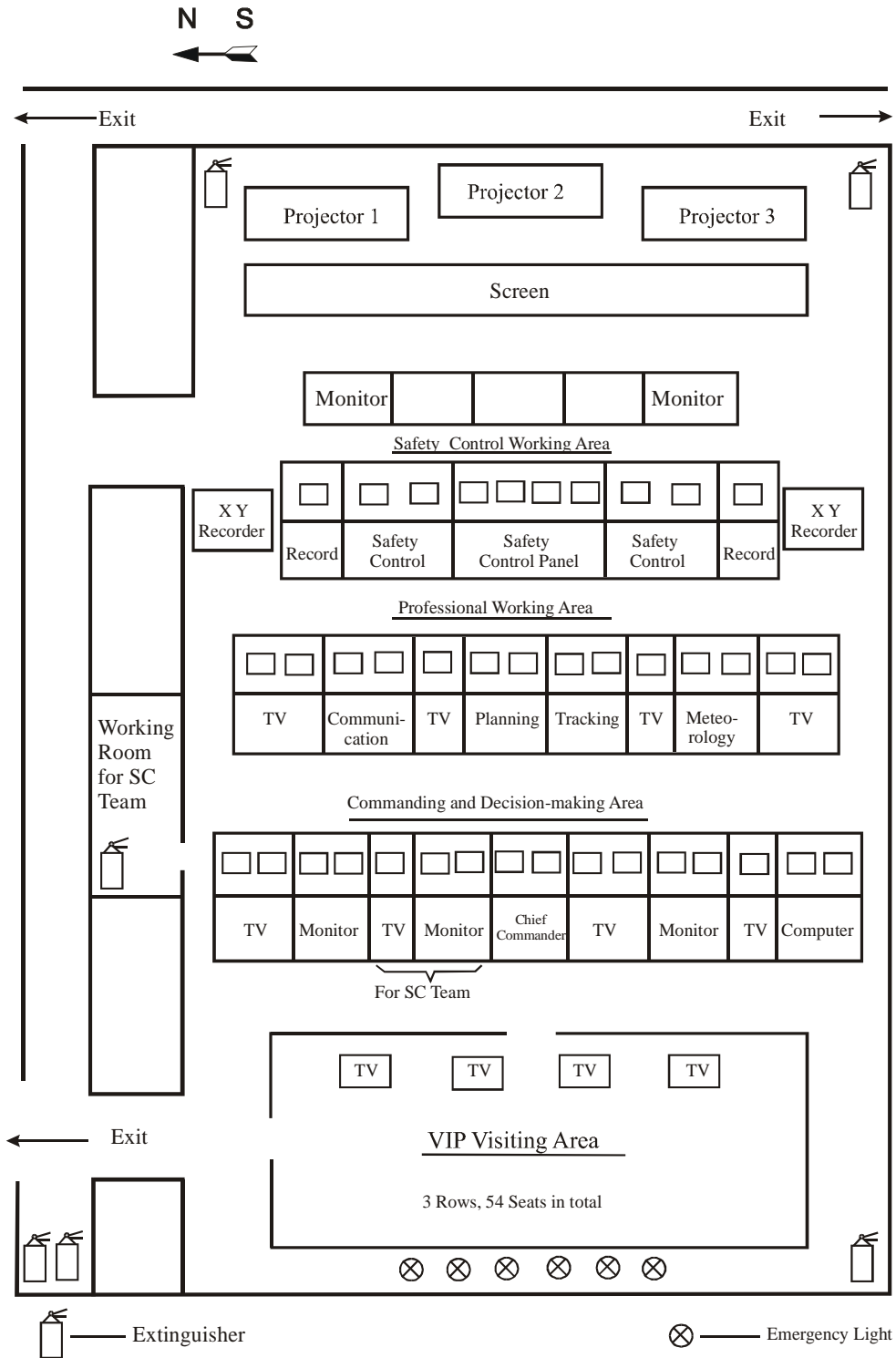
Figure 7-9 Layout of MCCC
