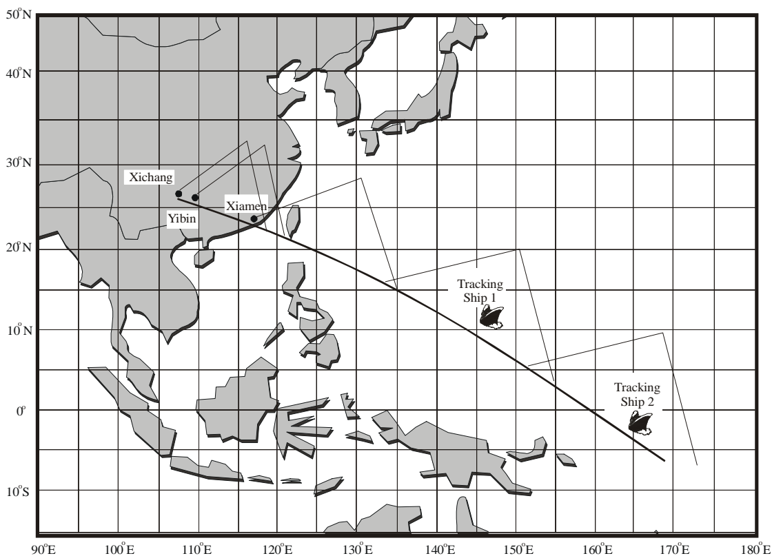
Figure 7-10 Tracking Stations
