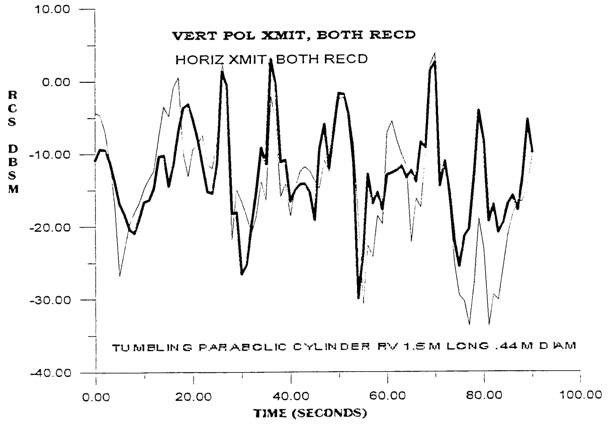
FIGURE 26a RCS vs aspect, aspect history, and RCS vs time for tumbling RV
