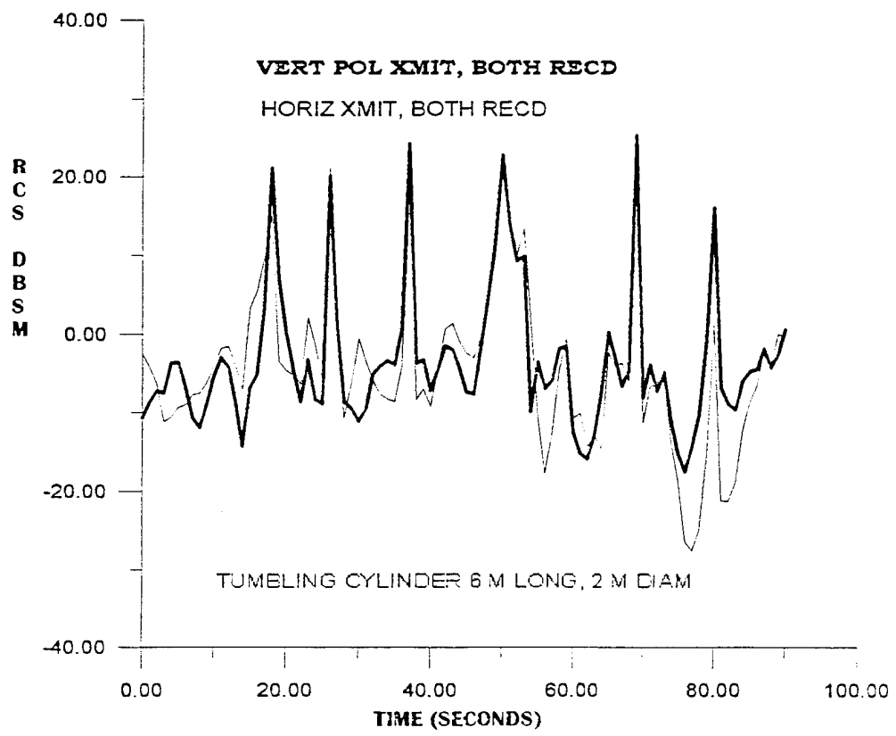
FIGURE 28a RCS vs aspect, aspect history, and RCS vs time for tumbling cylinder
