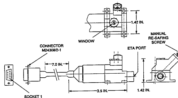
Figure 4. Safe-and-Arm Device
