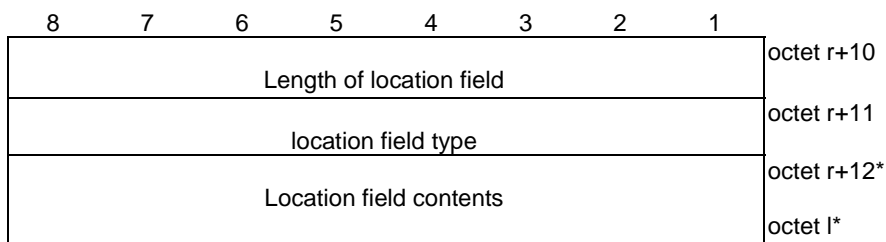
Figure 5.3.2.11c: Location field {entry type= WLAN location}
