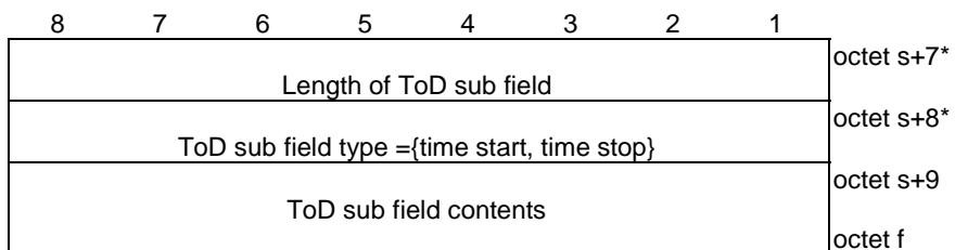
Figure 5.3.2.18: ToD sub field {field type = "time start" or "time stop"}
