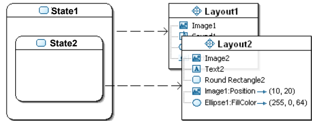
Figure 2. Presentation diagrams can be assigned to hierarchical states, new presentation elements can be added for substates or properties of existing elements be modified.
