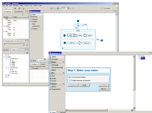
Figure 6. The GUI of GuiBuilder.
