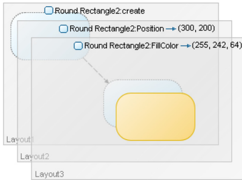
Figure 3. Stepwise modification of a presentation element through hierarchical presentation diagrams.
