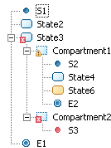
Figure 4. Problems are marked at the causing model elements.
