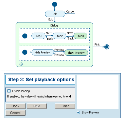
Figure 5. Simulations can be tracked in the model.
