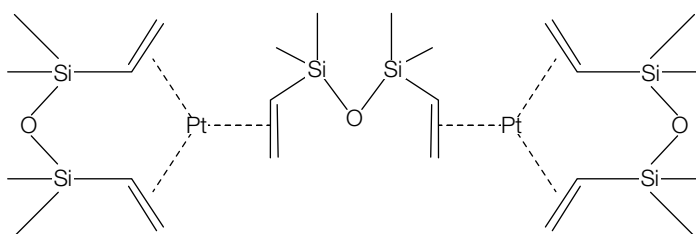
Karstedt's Catalyst
