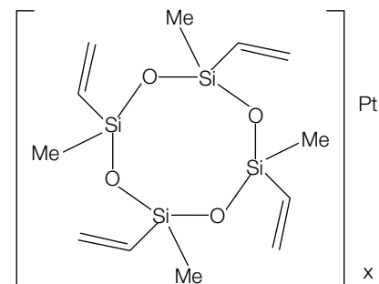
Ashby's Catalyst
