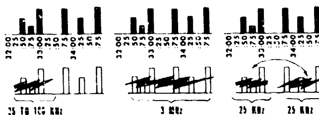
SPOT JAMMING BARRAGE JAMMING SWEEP JAMMING
