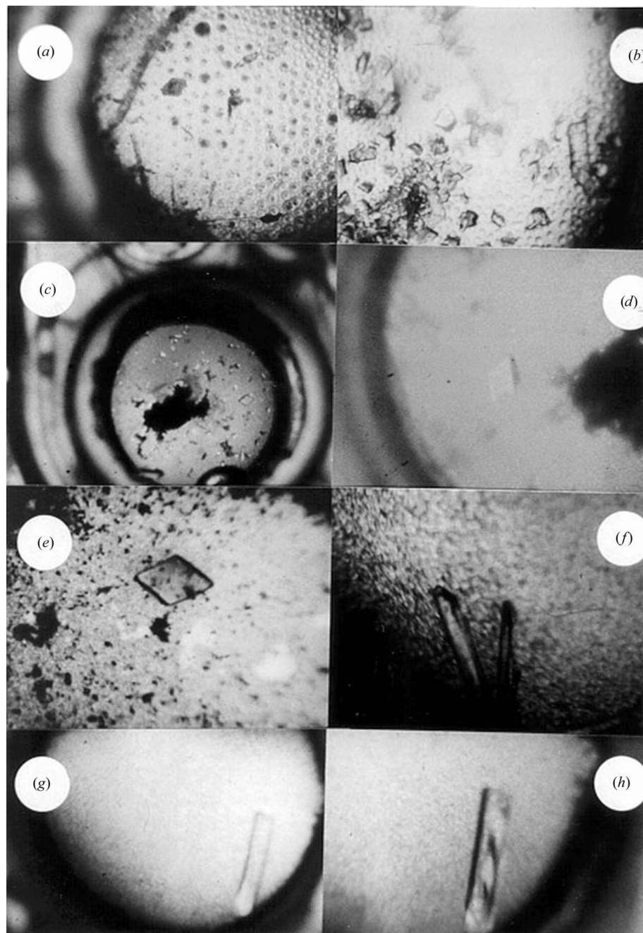
Figure 1 Crystallization of A31P. ( a )–( c ) Growth of a seed stock in microdialysis cells. ( d ), ( e ) Growth of lozenge-shaped crystals (space group C22_1 ) at pH 4.4 in cells to which seeds from the originally grown stock had been transferred. ( f )–( h ) Growth of rod-shaped crystals (space group C2 ) at pH 4.8 in cells to which seeds from the originally grown stock had been transferred.
