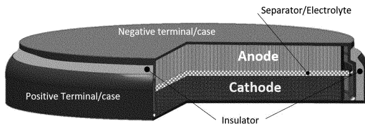
Figure 2. Components of a Button Cell or Coin Cell Battery
