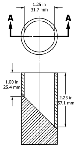
Figure 4. Small Parts Cylinder (16 CFR part 1501.4)
