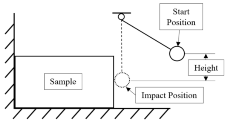
Figure 51. Example impact test with a swinging steel sphere
