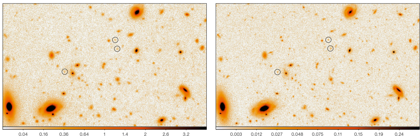
Figure 2. The centre of the deepest GOODS-S field as observed with HAWK-I is shown in the K -band (left) and with WFC3/IR in the H -band (right). The displayed area is 1 arcminute wide. Objects encircled have H \approx 26 mag and a colour ( H - K ) \approx 0.5 , typical of faint galaxies.
