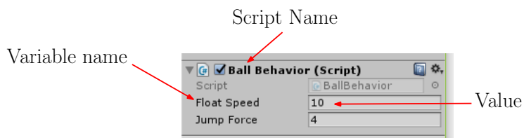
Fig. 2: Editing a public variable in the inspector.
