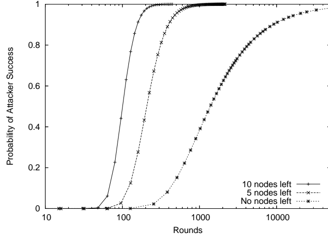
Fig. 3. Dynamic membership model: The probability of having less than ten and less than five nodes other than the initiator remaining in the system, and the probability of having no other nodes remaining, over time, where the system starts with n = 1,000 nodes.
