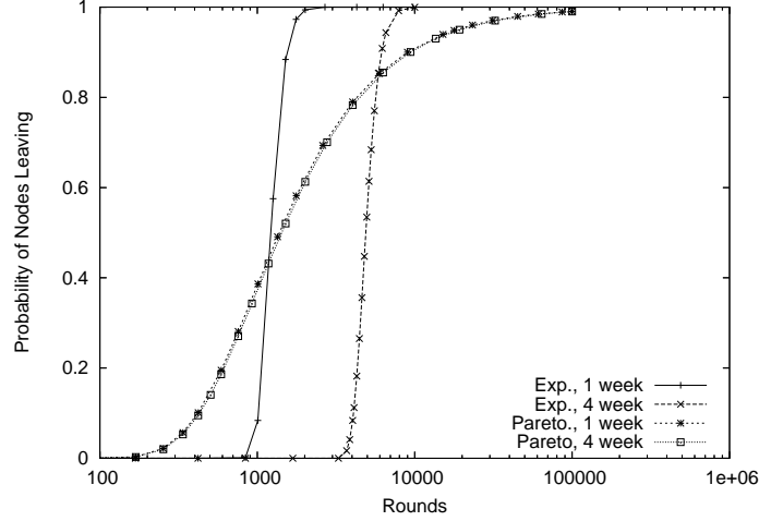
Fig. 1. Dynamic membership model: The intersection attack. The probability, for n = 1,000 nodes, of all nodes other than the initiator being intersected out of the set of possible initiators.
