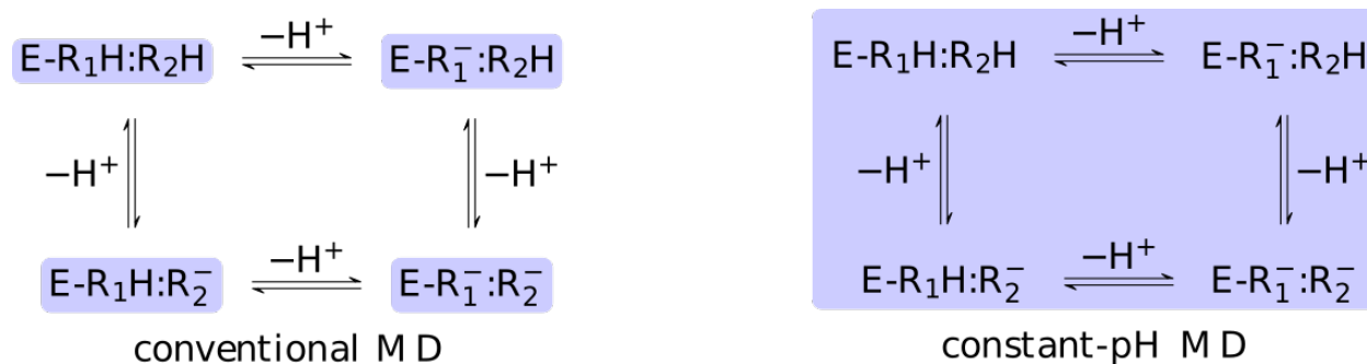
Figure 12: The core difference between conventional and constant-pH MD can be illustrated by a simple enzyme E with four protonation states describing the occupancy of two titratable residues, R_1 and R_2 . A conventional MD simulation handles the states separately (left panel). The relative importance of the states must be known beforehand or computed by other means. Conversely, a constant-pH MD simulation handles the states collectively and actively simulates interconversion (right panel). Determining the relative importance of the states is a direct result of the simulation.
