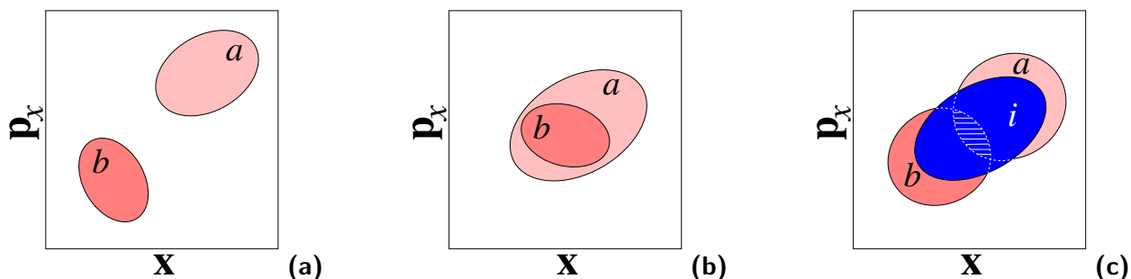
Figure 8: Convergence of an FEP calculation. If the ensembles representative of states a and b are too disparate, equation (66) will not converge (a) . If, in sharp contrast, the configurations of state b form a subset of the ensemble of configurations characteristic of state a , the simulation is expected to converge (b) . The difficulties reflected in case (a) may be alleviated by the introduction of mutually overlapping intermediate states that connect a to b (c) . It should be mentioned that in practice, the kinetic contribution, \mathcal{T}(\mathbf{p}_x) , is assumed to be identical for state a and state b .
