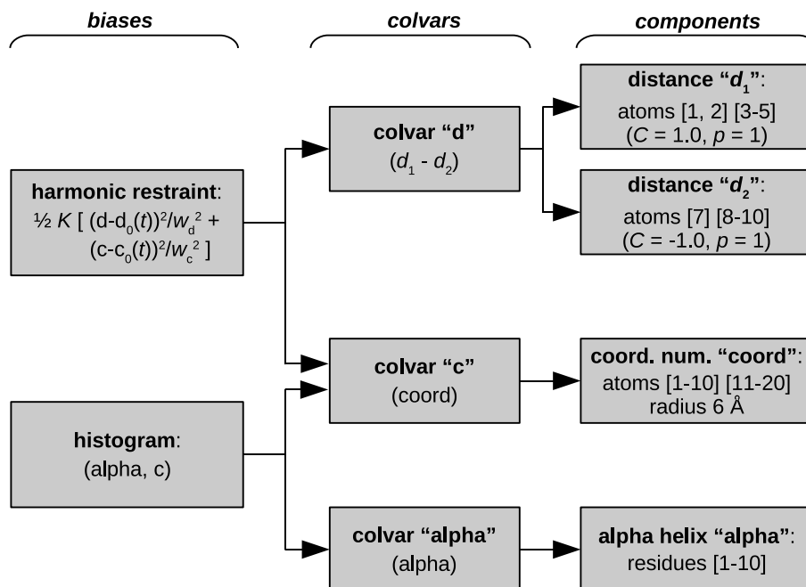
Figure 6: Graphical representation of a Colvars configuration. The colvar called “ d ” is defined as the difference between two distances: the first distance ( d_1 ) is taken between the center of mass of atoms 1 and 2 and that of atoms 3 to 5, the second ( d_2 ) between atom 7 and the center of mass of atoms 8 to 10. The difference d = d_1 - d_2 is obtained by multiplying the two by a coefficient C = +1 or C = -1 , respectively. The colvar called “ c ” is the coordination number calculated between atoms 1 to 10 and atoms 11 to 20. A harmonic restraint is applied to both d and c : to allow using the same force constant K , both d and c are scaled by their respective fluctuation widths w_d and w_c . A third colvar “alpha” is defined as the \alpha -helical content of residues 1 to 10. The values of “ c ” and “alpha” are also recorded throughout the simulation as a joint 2-dimensional histogram.
