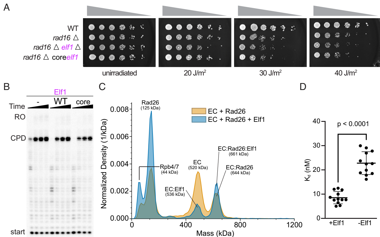
Fig. 2. Elf1 enhances interactions between Pol II and Rad26. (A) Deletion of Elf1 leads to UV sensitivity and can be rescued by Elf1 core. (B) Elf1, or Elf1 core have no effect on the stalling of Pol II at a CPD lesion. Time points were 0.3, 1, 3, and 10 min. (C) Mass photometry of EC + Rad26 in the absence or presence of Elf1. Peak identities and predicted molecular weights are indicated. (D) K_d s for the interaction between Pol II (EC) stalled at a CPD lesion and Rad26 in the absence or presence of Elf1 were determined from multiple repeats of the experiment in (C). P < 0.0001 , two-tailed Student’s t test. Data are mean and SD ( n = 12 ). The final Elf1 concentrations were 1 \mu\text{M} (B) and 0.5 \mu\text{M} (C). All assays were performed at least three times independently.
