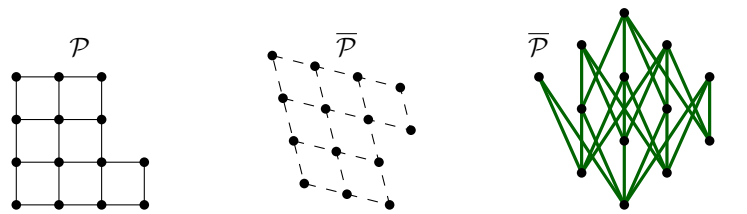
Figure 3. The Hasse diagram of a two-dimensional poset \mathcal{P} , its complement \overline{\mathcal{P}} as a set of points in \mathbb{R}^2 , and the Hasse diagram of \overline{\mathcal{P}} .
