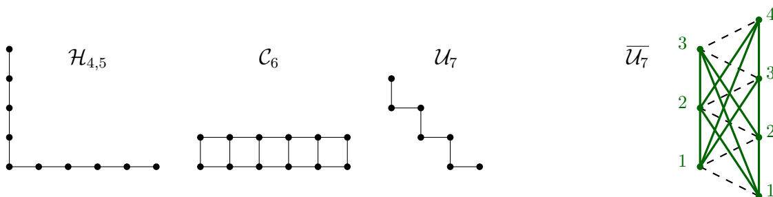
Figure 2. Two-dimensional posets \mathcal{H}_{4,5} , \mathcal{C}_6 , \mathcal{U}_7 and a complement of \mathcal{U}_7 .
